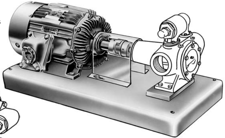
SERIES 4195 Pumps with “D” Drive “AS”, “AK” and “AL” Sizes
