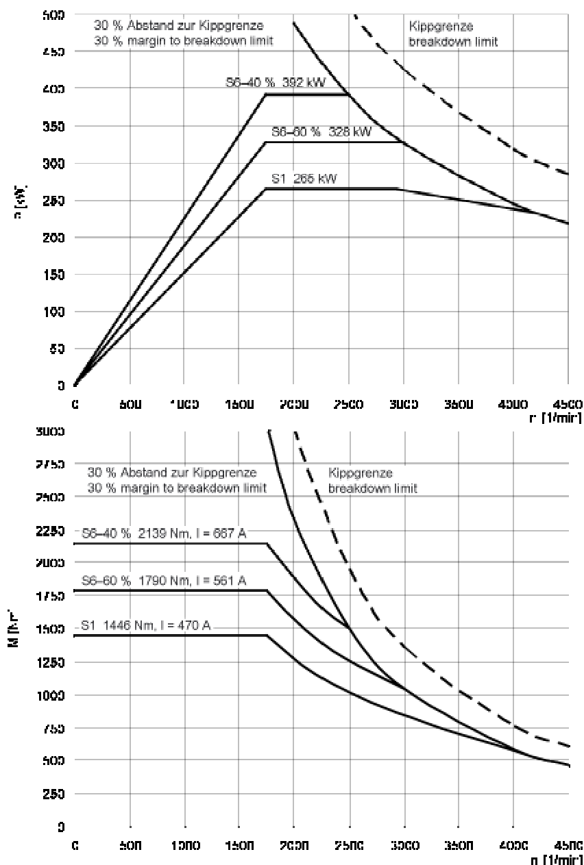
Figure 3-21 MASTERDRIVES VC, 1PL6228-□□F□□
