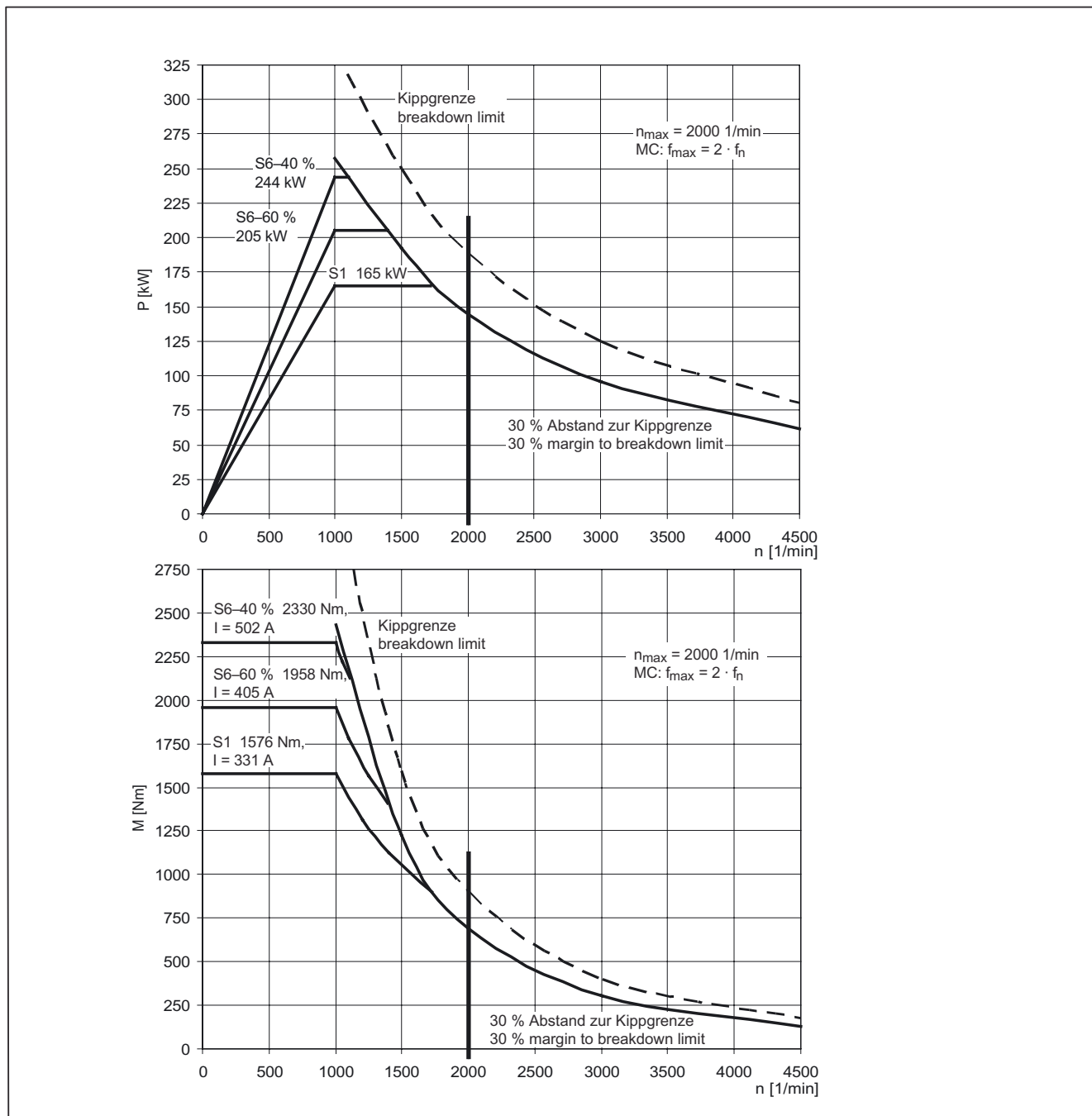
Figure 3-77 MASTERDRIVES MC, 1PL6228-□□D□□
