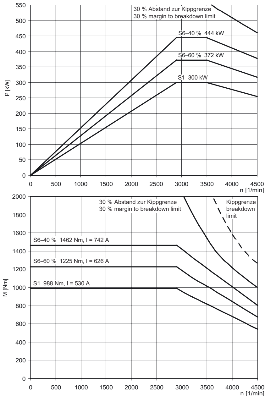
Figure 3-58 MASTERDRIVES VC, 1PL6228-□□L□□
