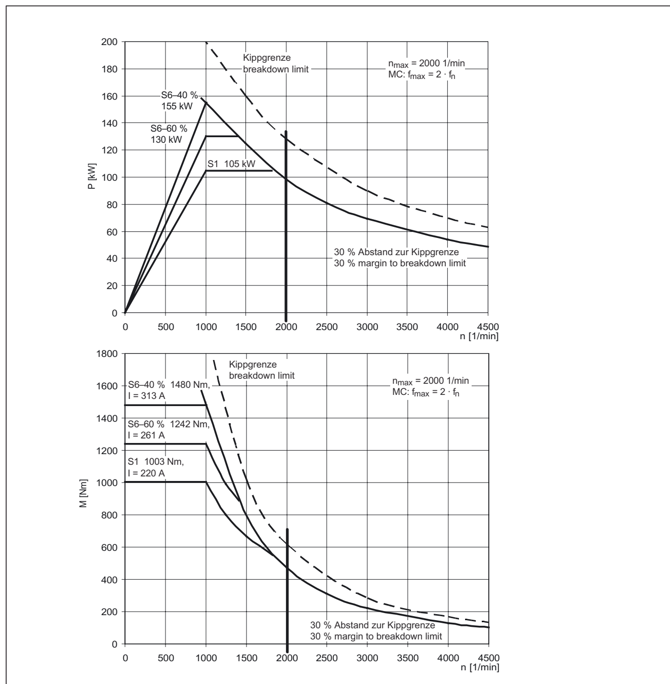
Figure 3-75 MASTERDRIVES MC, 1PL6224-□□D□□
