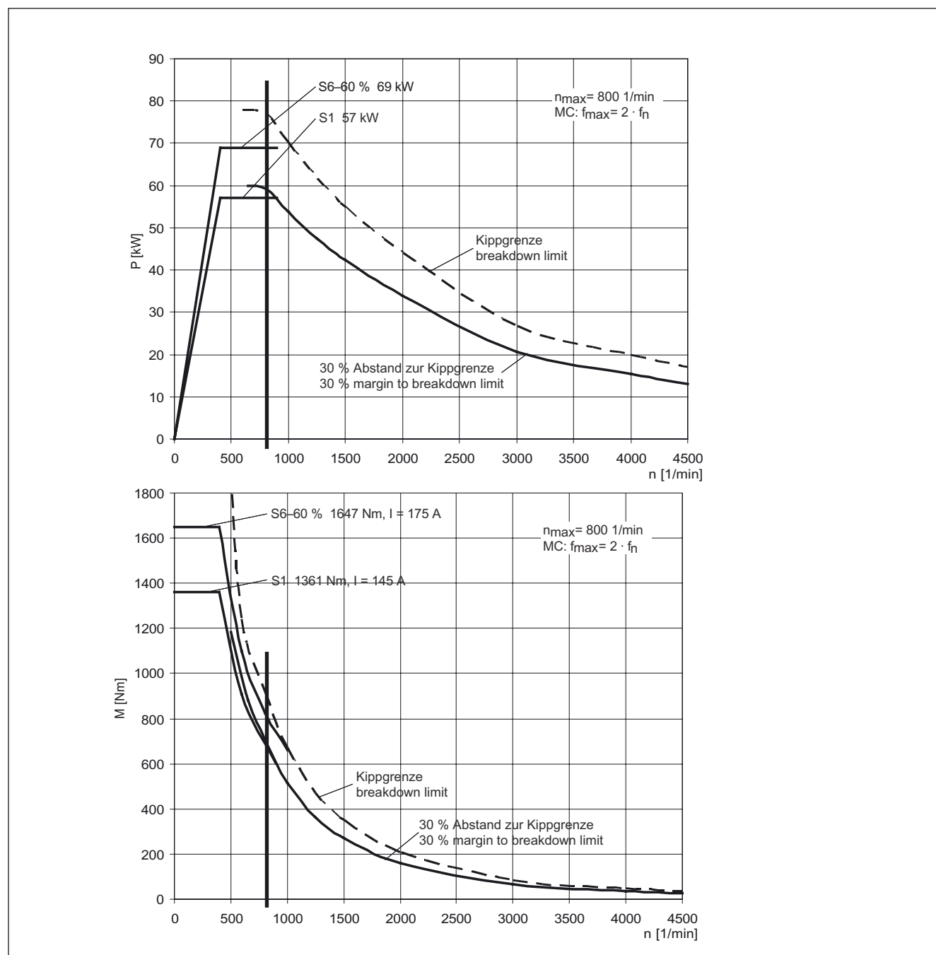
Figure 3-71 MASTERDRIVES MC, 1PL6226-□□B□□
