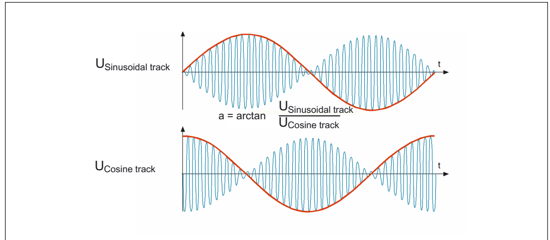
Figure 4-5 Resolver output signals
