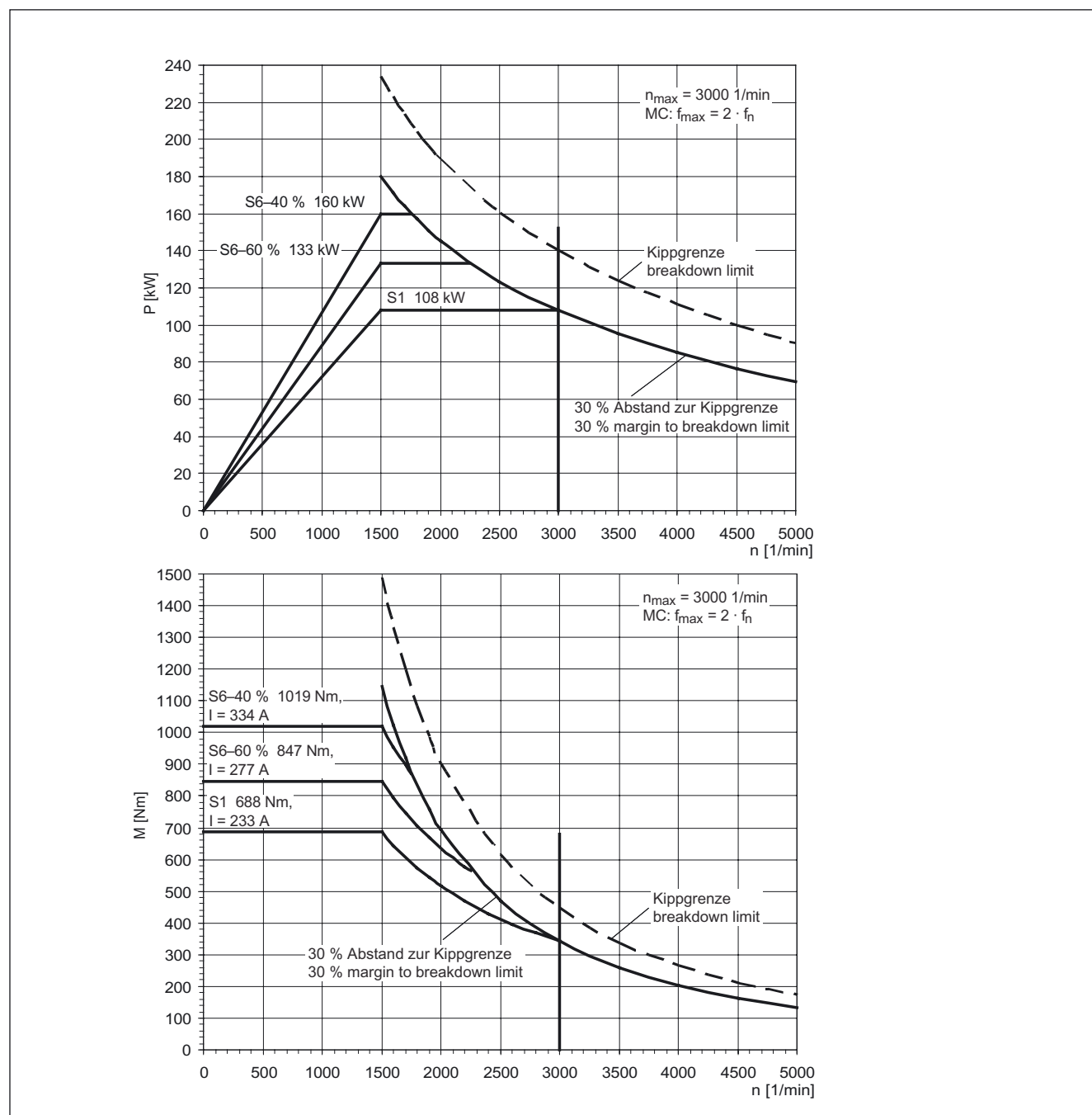
Figure 3-79 MASTERDRIVES MC, 1PL6186-□□F□□
