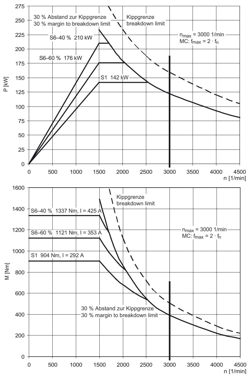
Figure 3-80 MASTERDRIVES MC, 1PL6224-□□F□□
