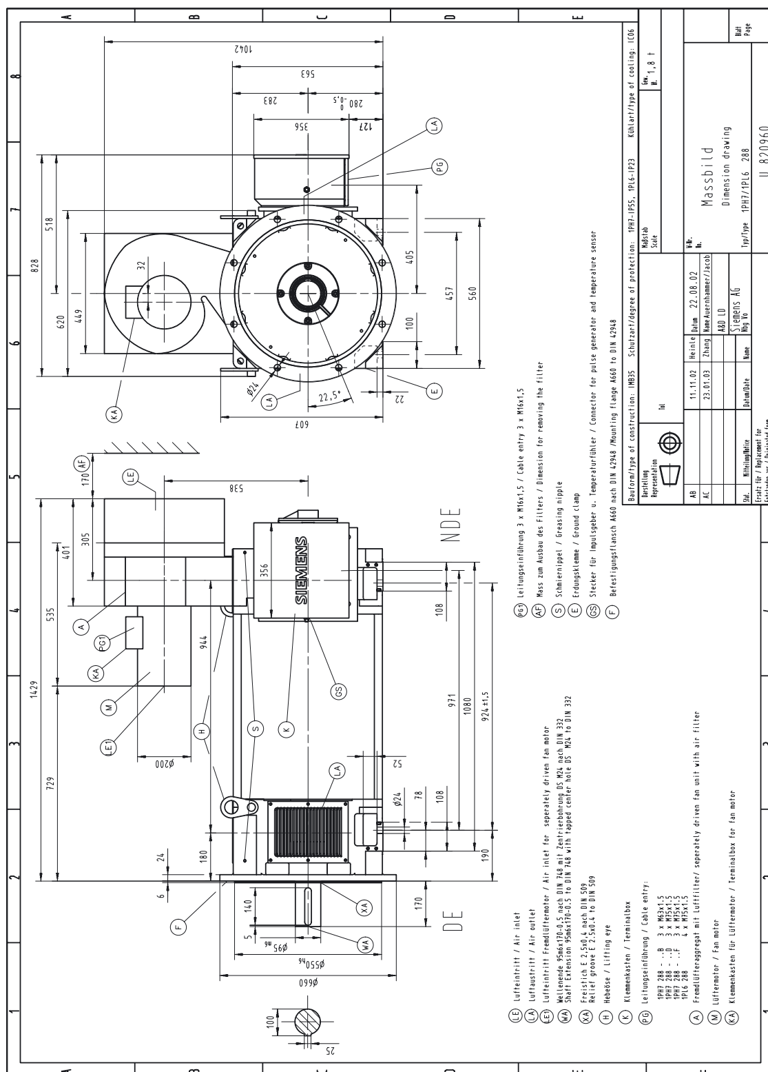
Figure 5-72 1PL6288, air flow direction NDE→DE, filter, U820960
