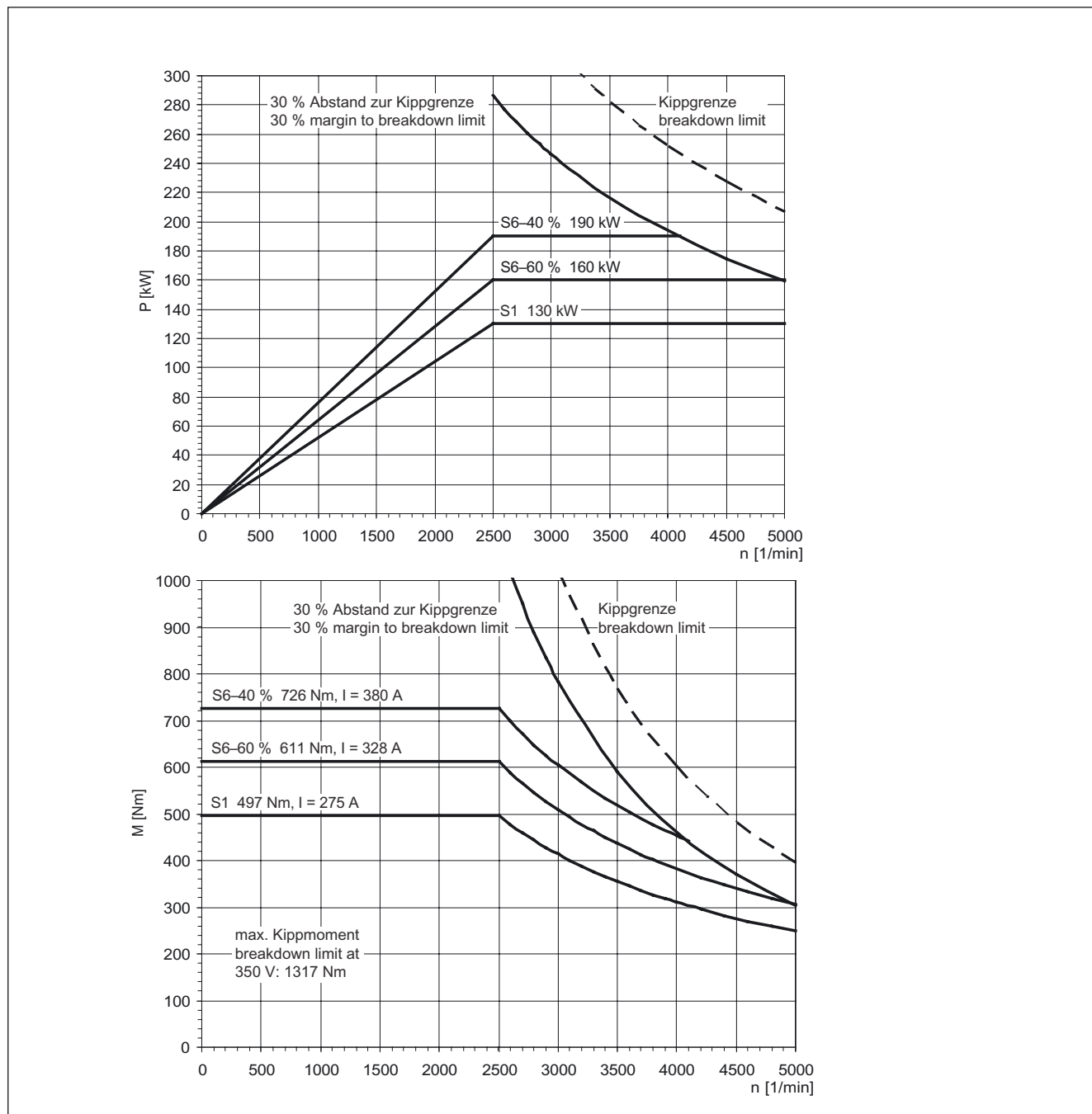
Figure 3-84 MASTERDRIVES MC, 1PL6186-□□L□□
