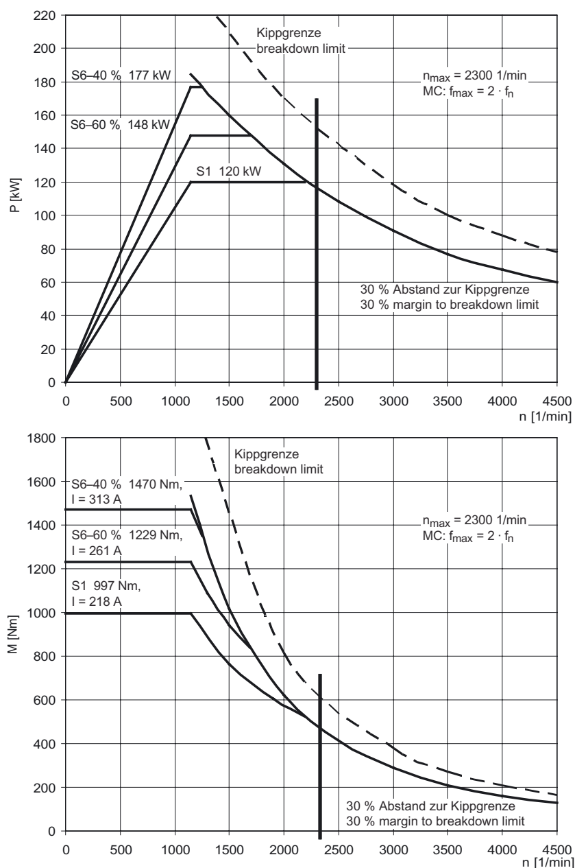
Figure 3-95 MASTERDRIVES MC, 1PL6224-□□D□□
