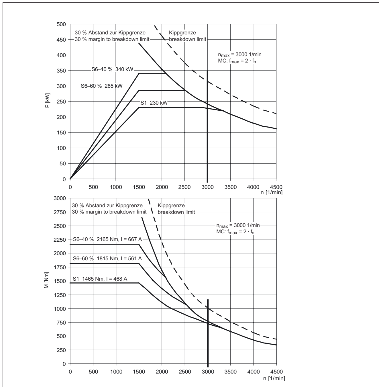
Figure 3-82 MASTERDRIVES MC, 1PL6228-□□F□□
