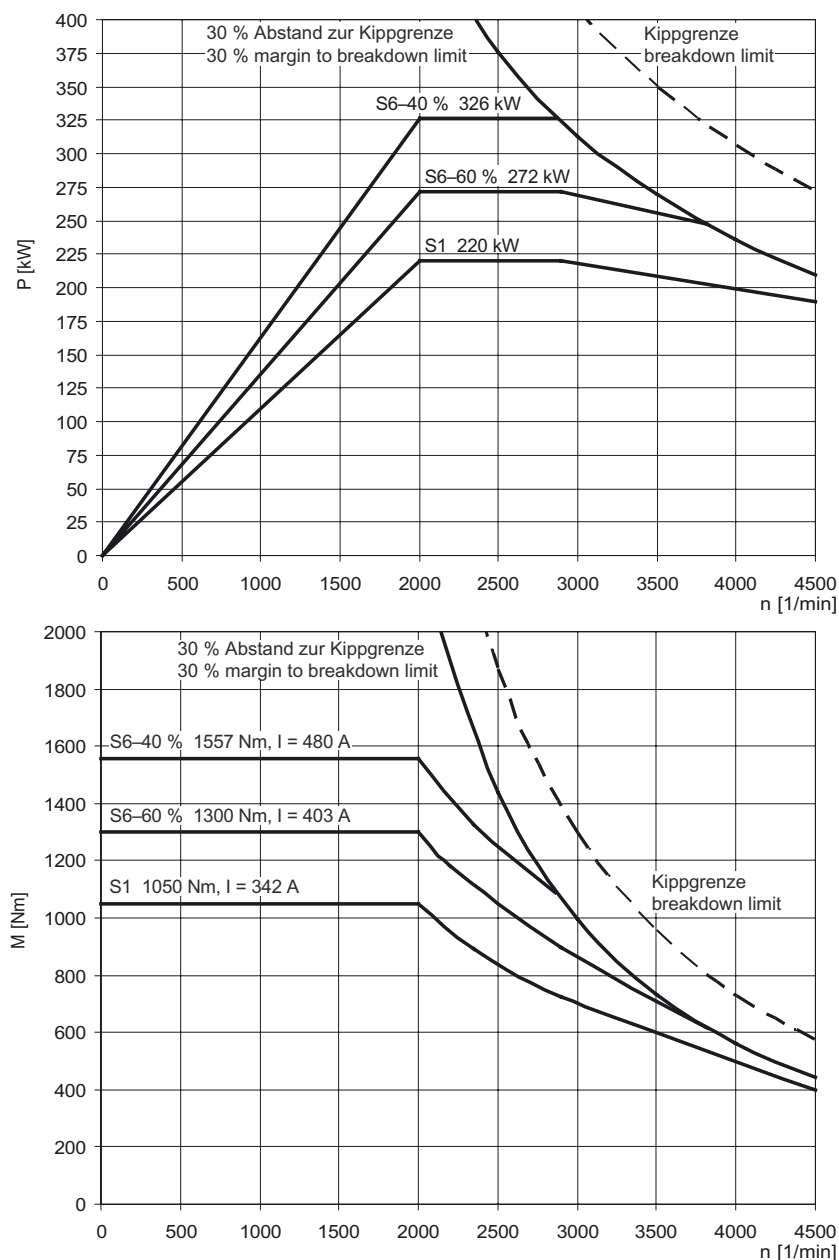
Figure 3-49 MASTERDRIVES VC, 1PL6226-□□F□□
