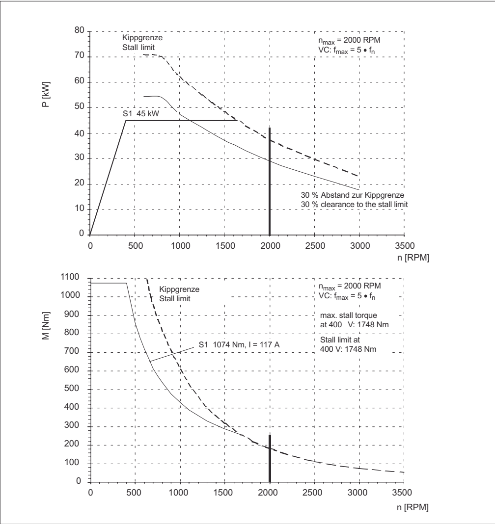
Figure 3-3 MASTERDRIVES VC, 1PL6224-□□B□□
