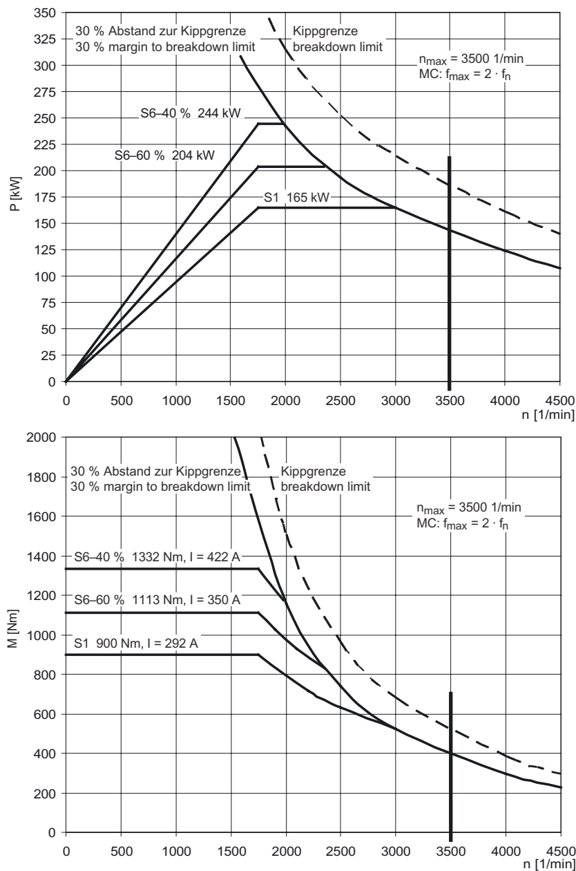
Figure 3-100 MASTERDRIVES MC, 1PL6224-□□F□□
