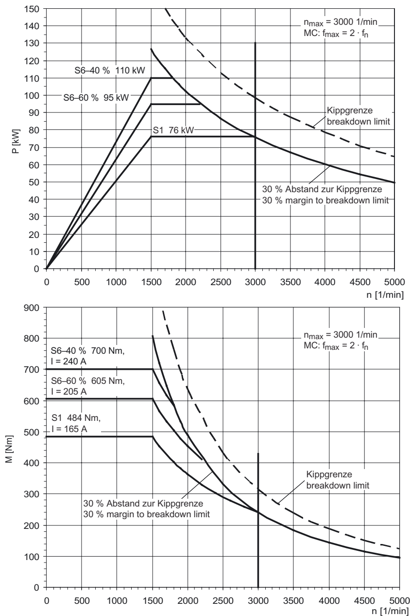
Figure 3-78 MASTERDRIVES MC, 1PL6184-□□F□□
