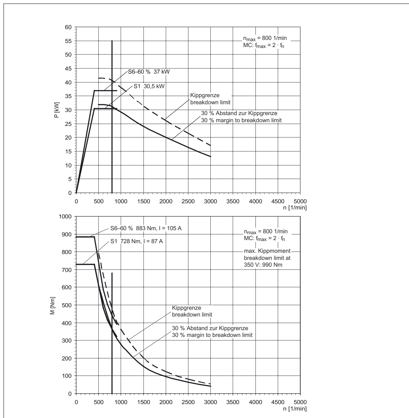
Figure 3-69 MASTERDRIVES MC, 1PL6186-□□B□□
