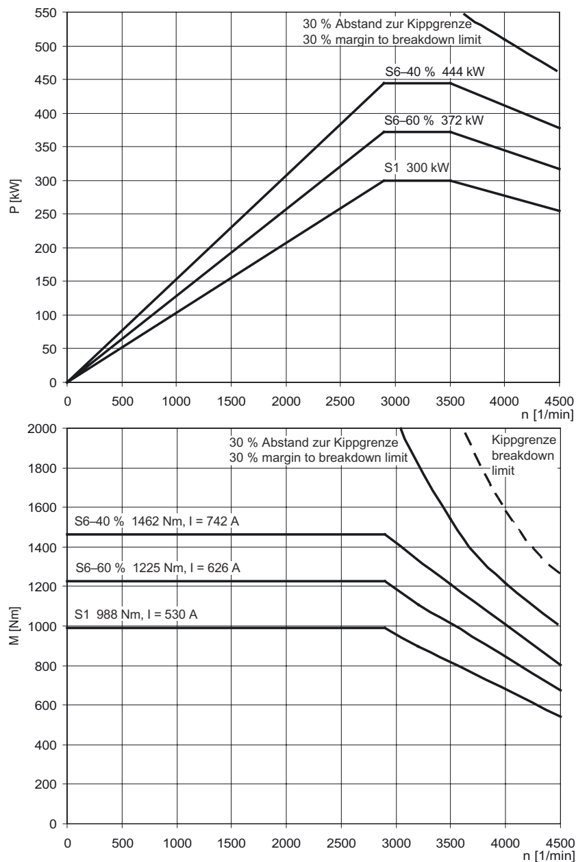
Figure 3-29 MASTERDRIVES VC, 1PL6228-□□L□□
