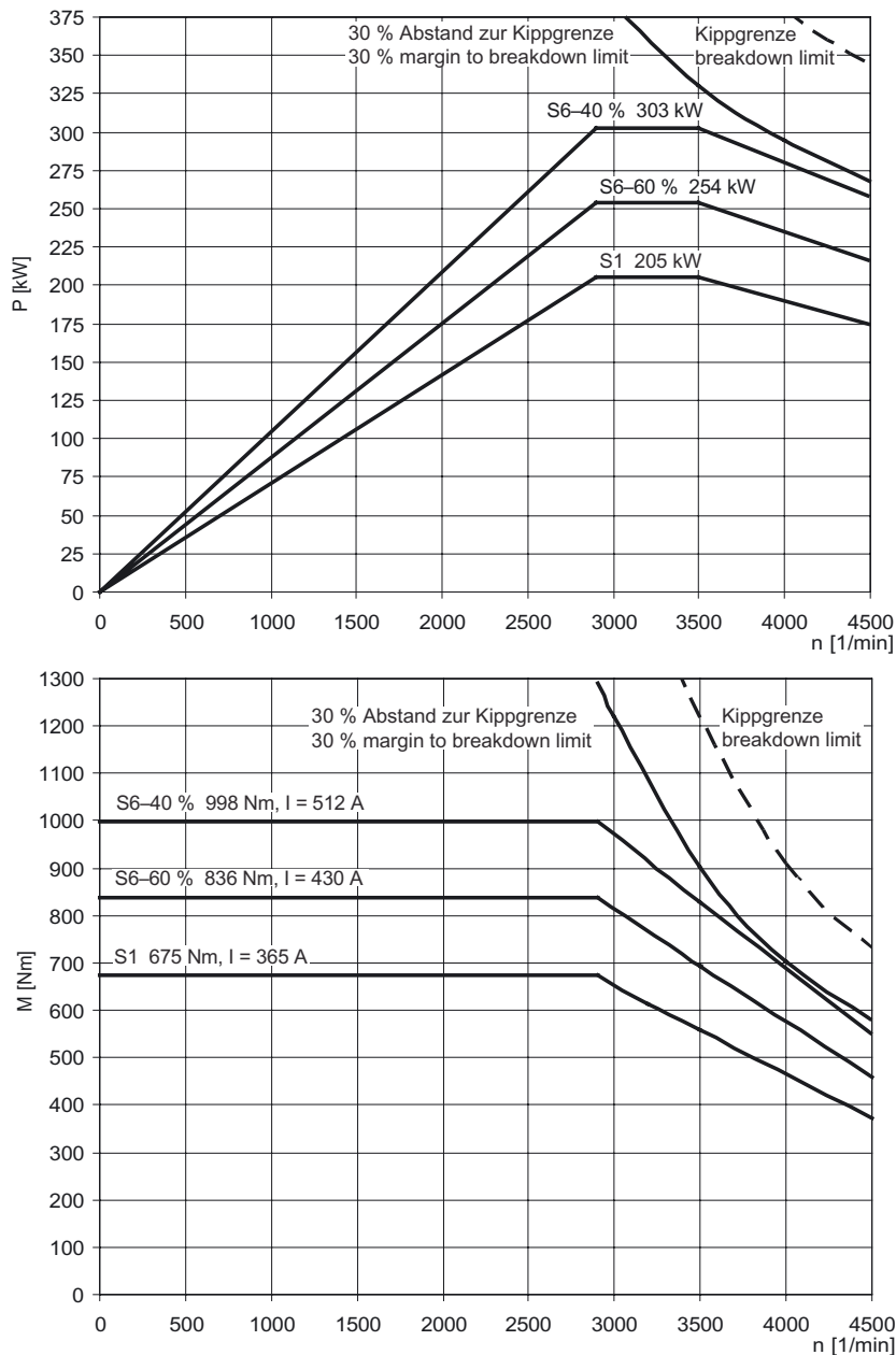
Figure 3-56 MASTERDRIVES VC, 1PL6224-□□L□□
