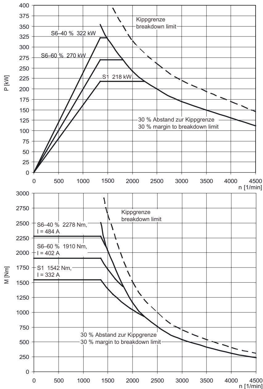
Figure 3-42 MASTERDRIVES VC, 1PL6228-□□D□□
