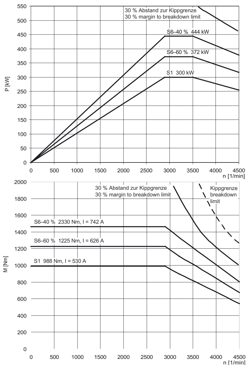
Figure 3-107 MASTERDRIVES MC, 1PL6228-□□L□□
