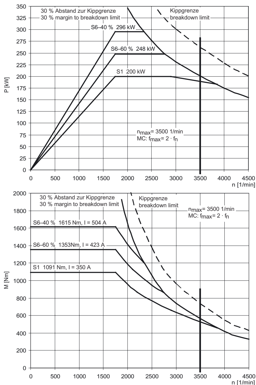
Figure 3-101 MASTERDRIVES MC, 1PL6226-□□F□□
