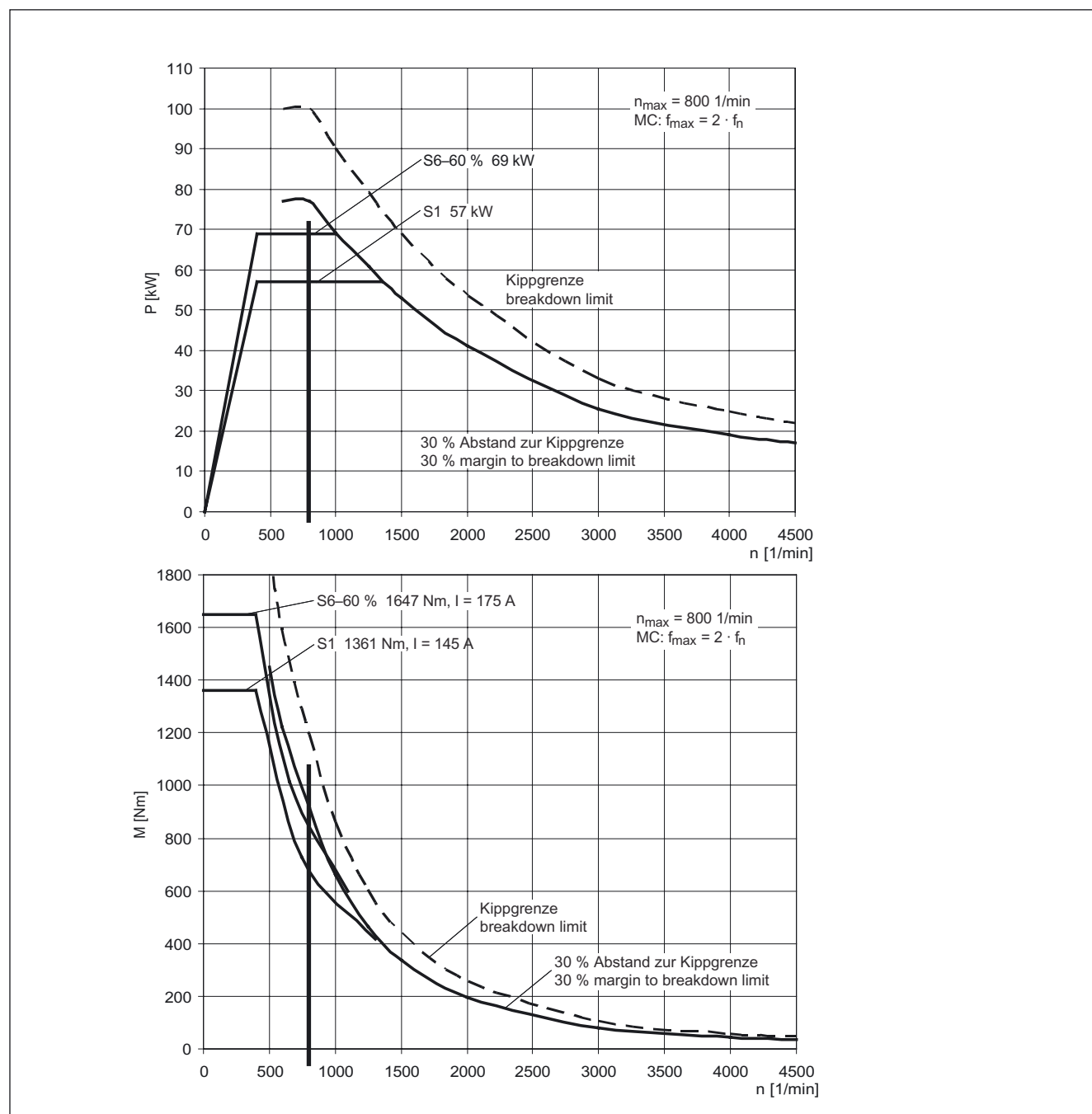
Figure 3-91 MASTERDRIVES MC, 1PL6226-□□B□□
