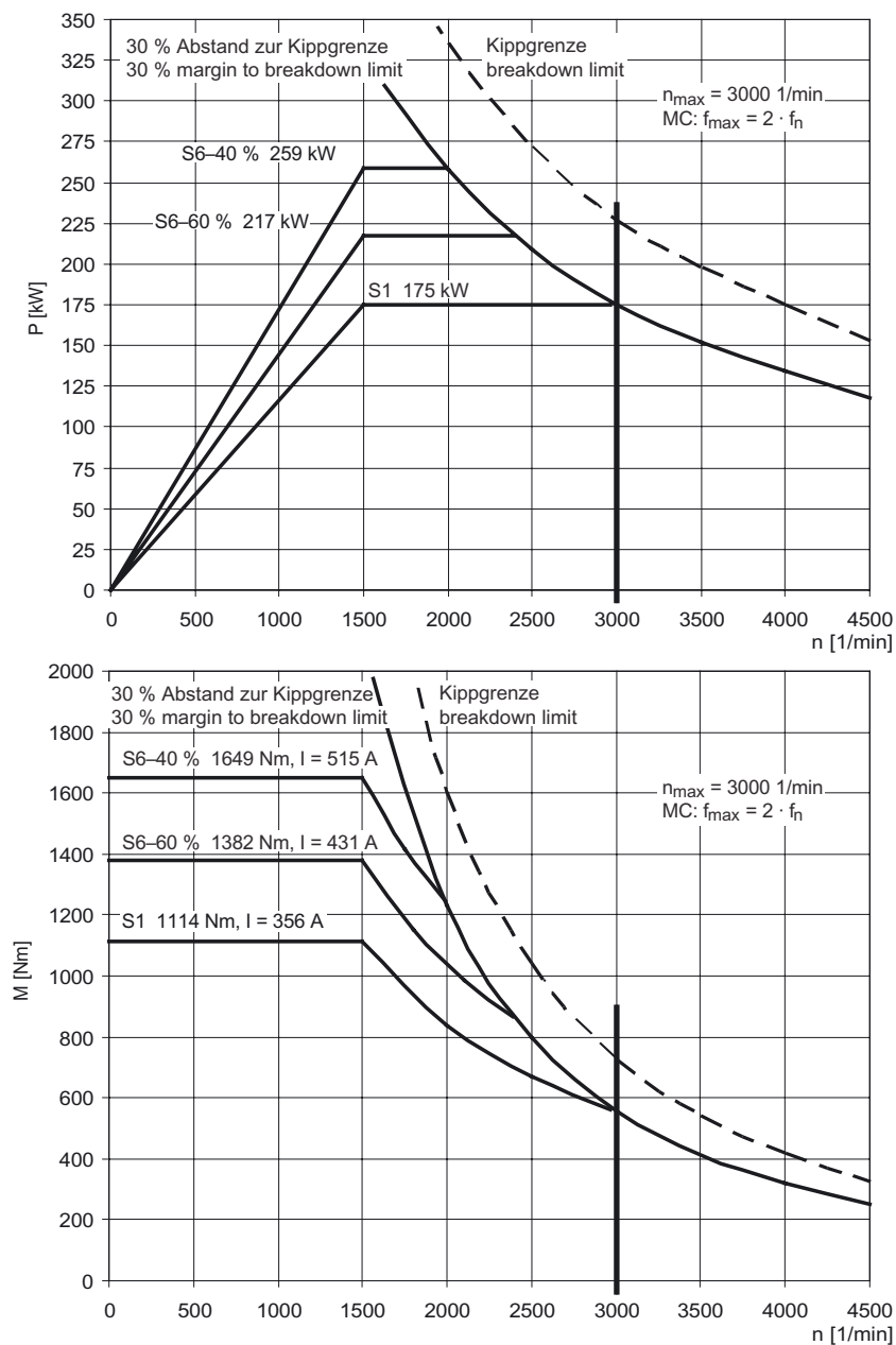
Figure 3-81 MASTERDRIVES MC, 1PL6226-□□F□□
