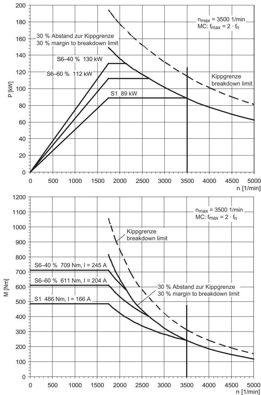
Figure 3-98 MASTERDRIVES MC, 1PL6184-□□F□□
