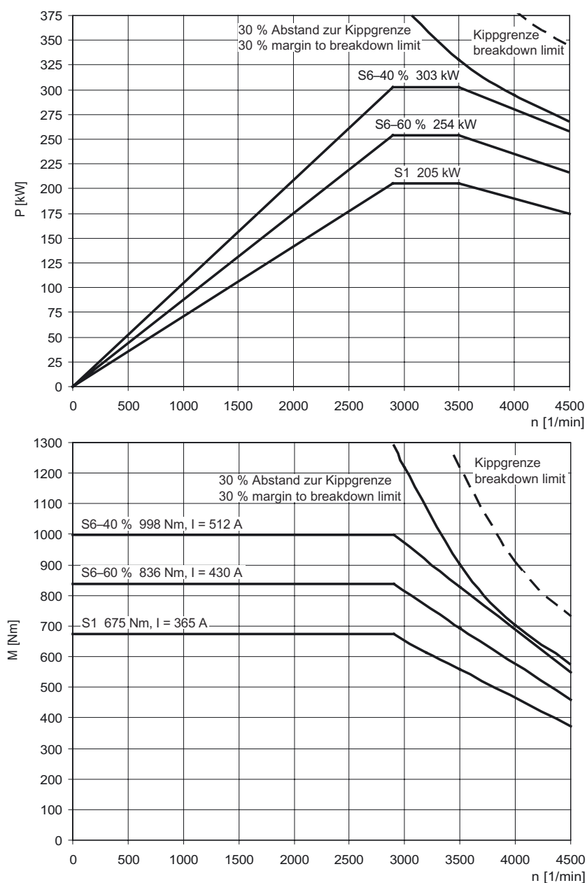
Figure 3-27 MASTERDRIVES VC, 1PL6224-□□L□□
