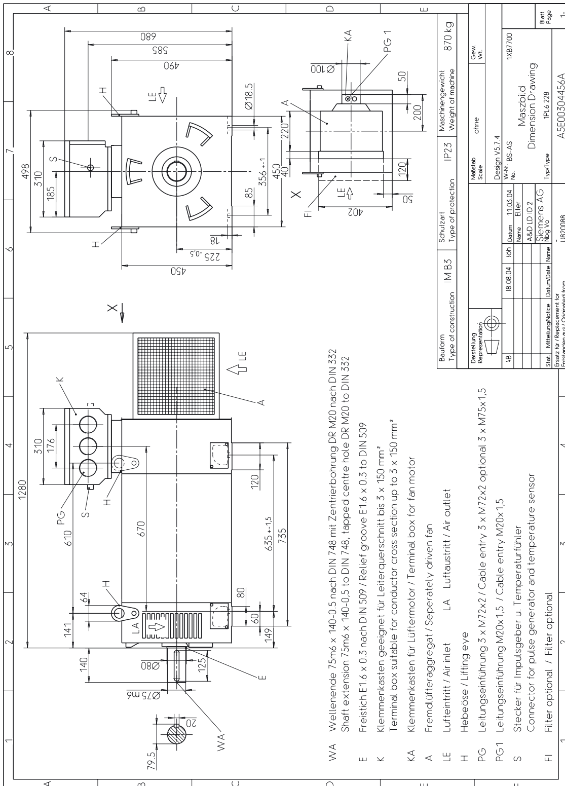
Figure 5-24 1PL6228-D-L, air flow direction NDE→DE, A5E00304456A
