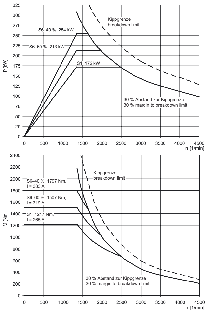
Figure 3-41 MASTERDRIVES VC, 1PL6226-□□D□□
