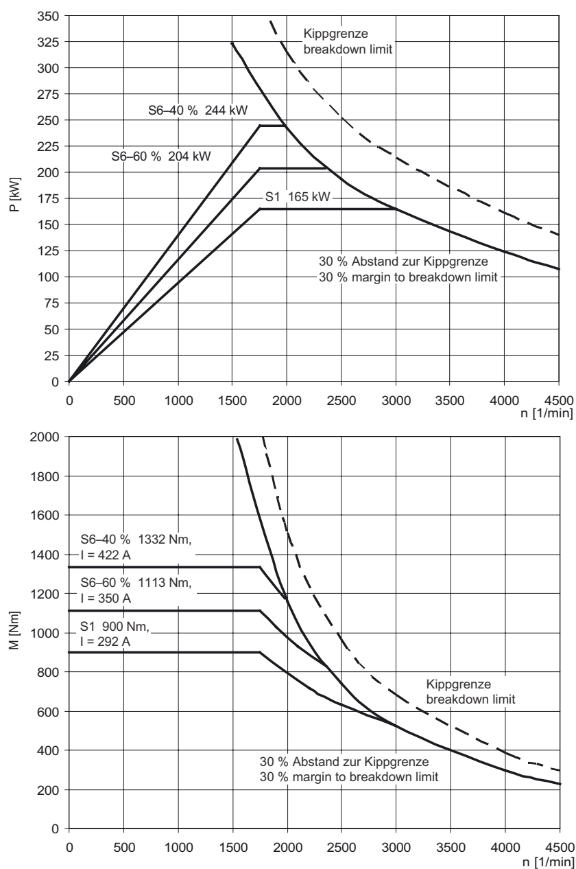
Figure 3-19 MASTERDRIVES VC, 1PL6224-□□F□□
