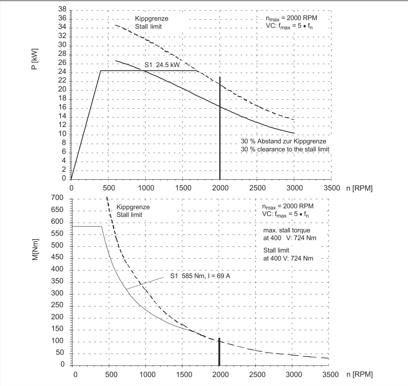
Figure 3-1 MASTERDRIVES VC, 1PL6184-□□B□□
