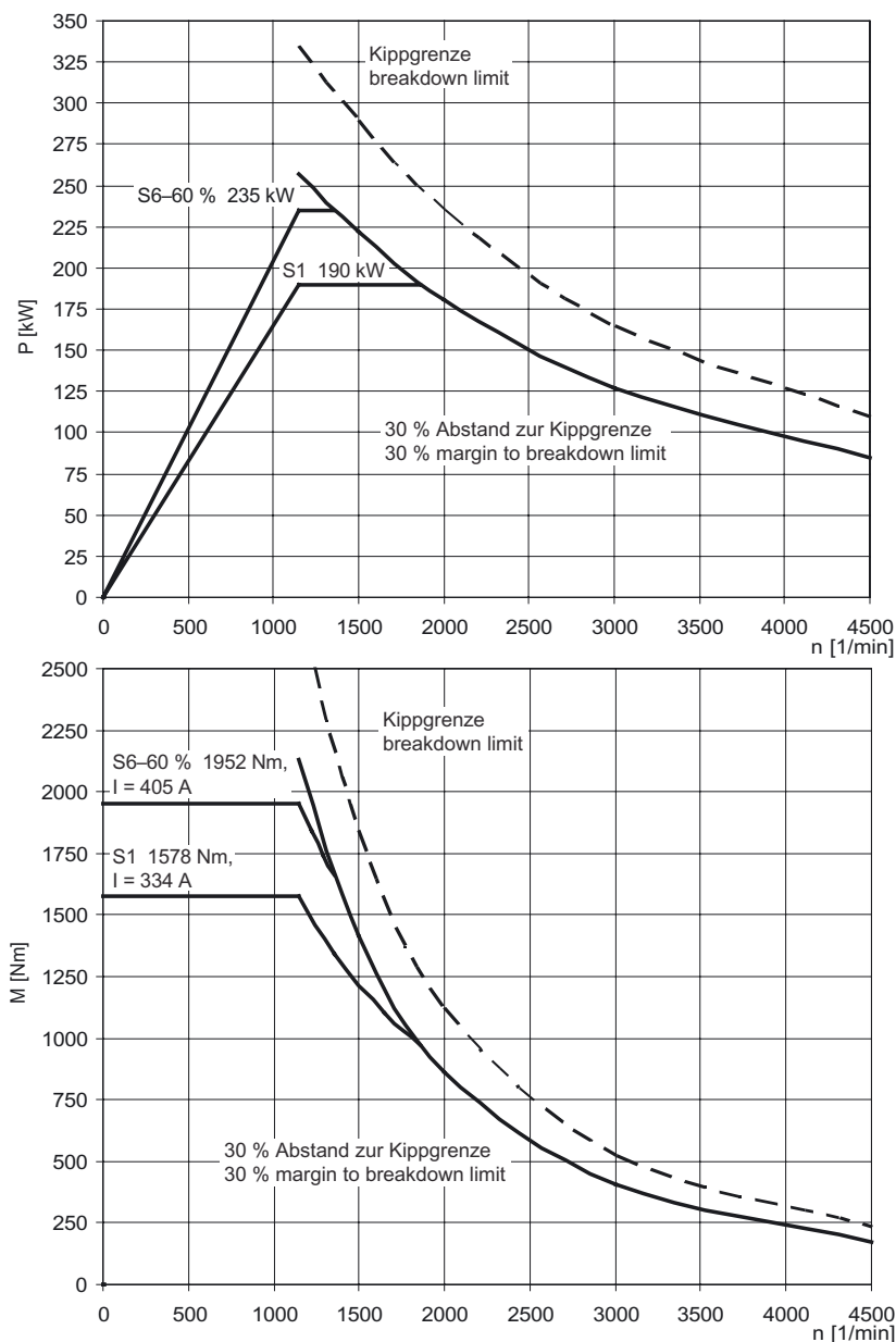
Figure 3-13 MASTERDRIVES VC, 1PL6228-□□D□□
