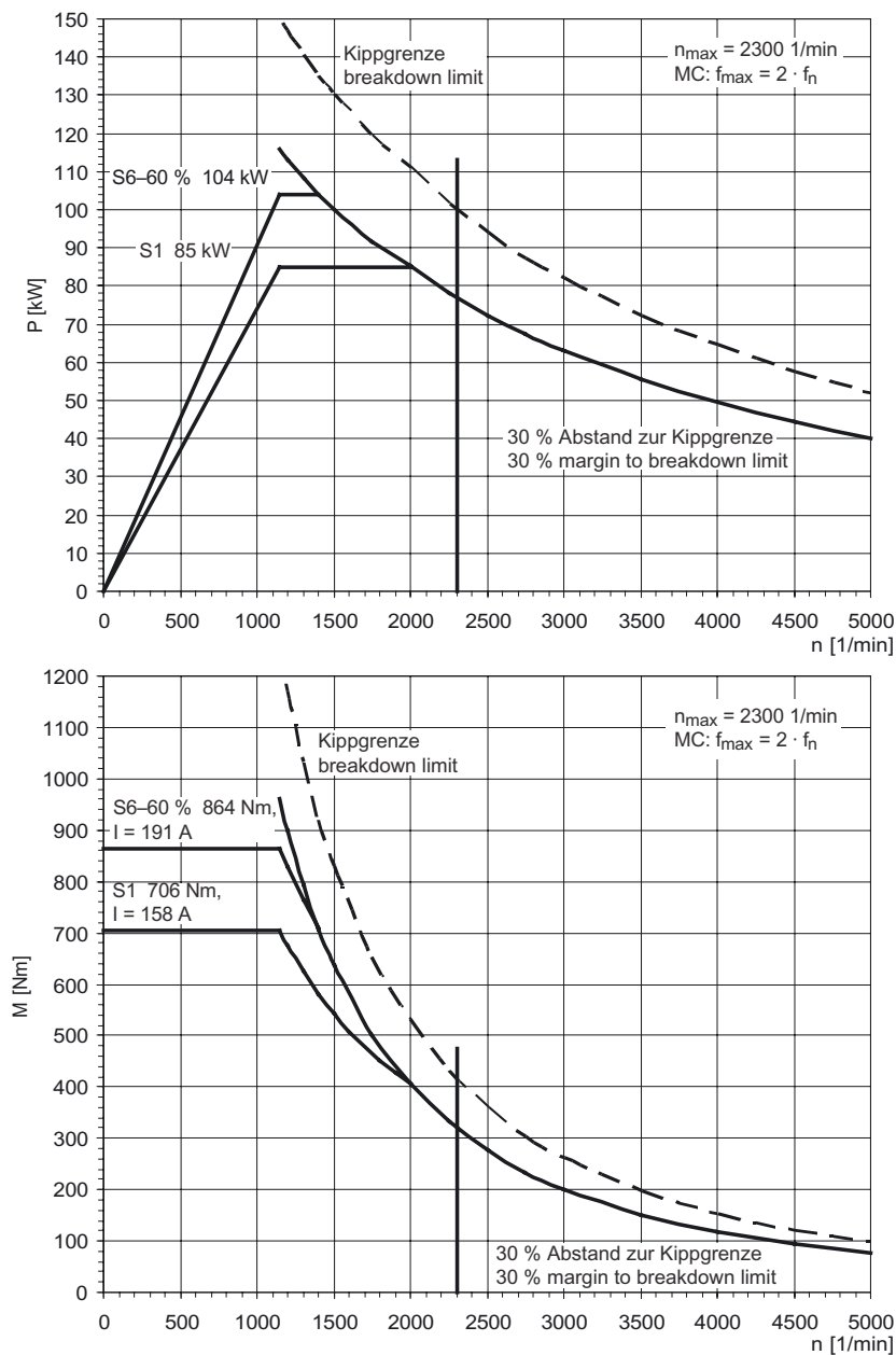
Figure 3-94 MASTERDRIVES MC, 1PL6186-□□D□□
