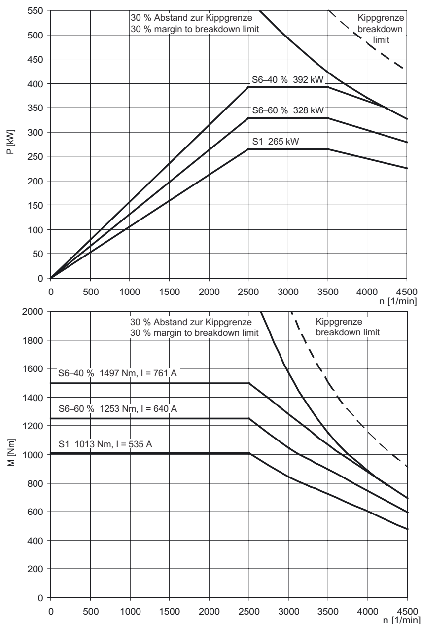
Figure 3-87 MASTERDRIVES MC, 1PL6228-□□L□□
