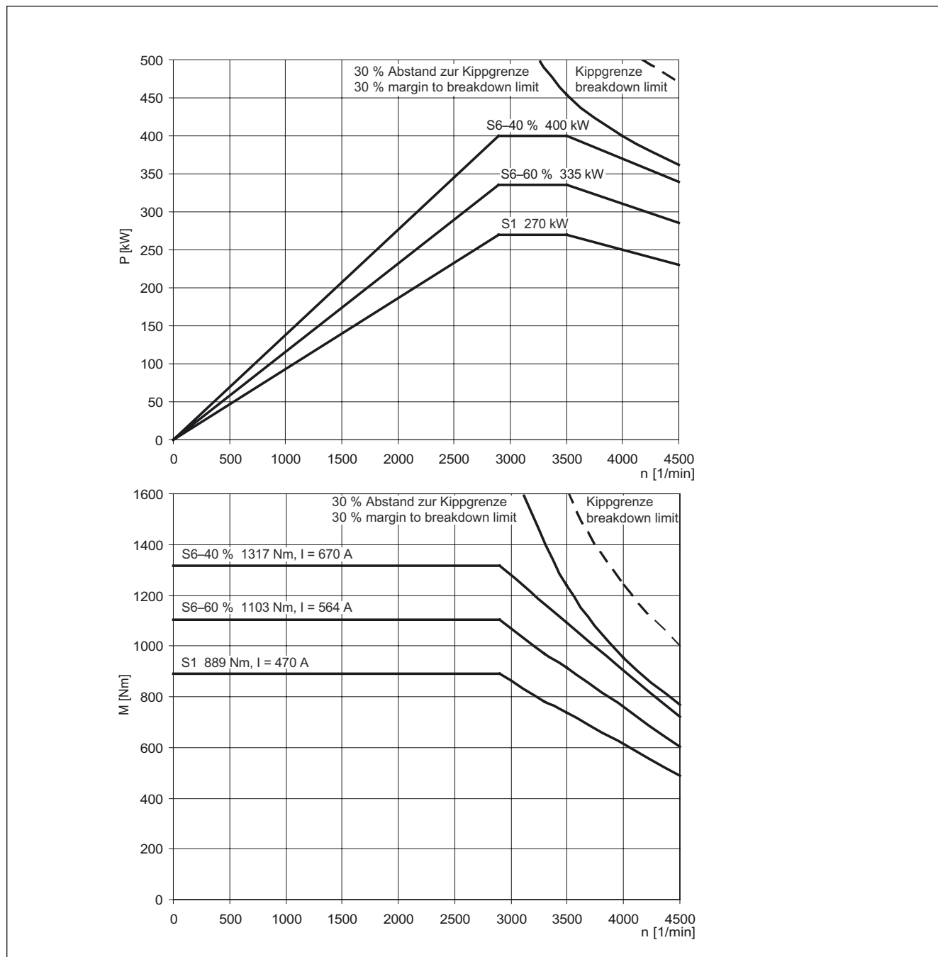
Figure 3-106 MASTERDRIVES MC, 1PL6226-□□L□□
