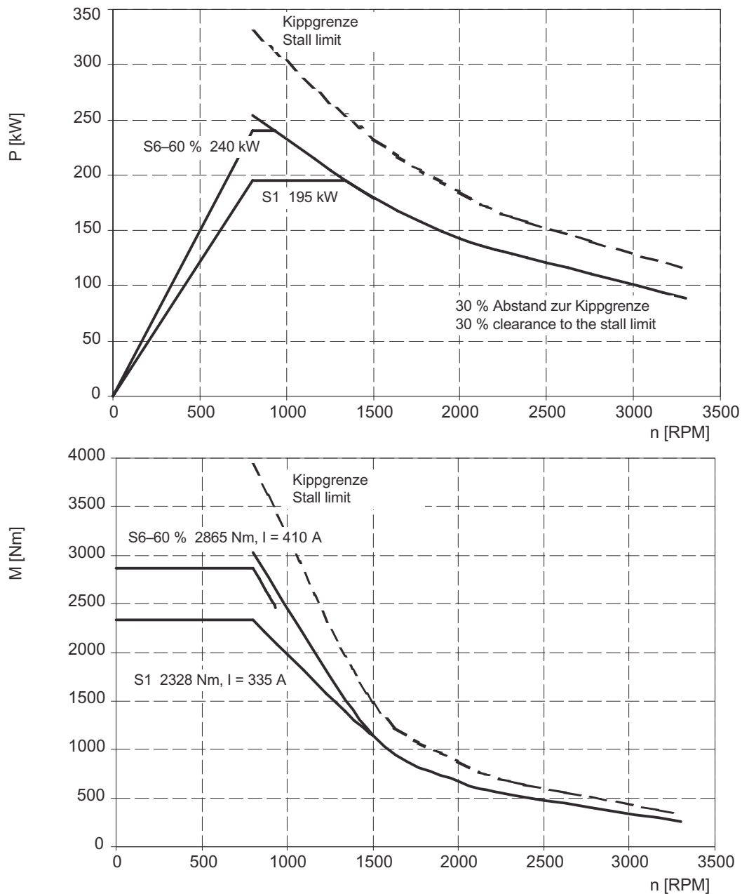
Figure 3-6 MASTERDRIVES VC, 1PL6284-□□C□□
