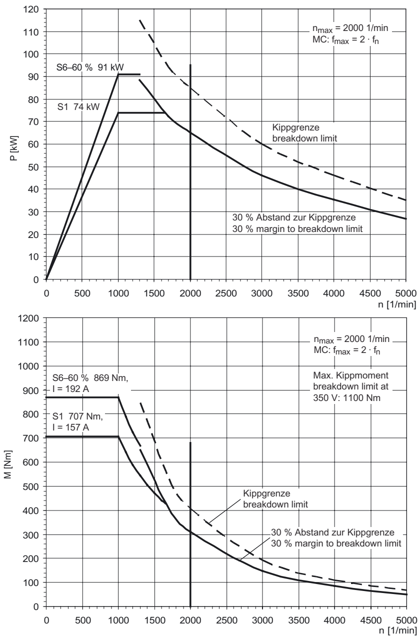
Figure 3-74 MASTERDRIVES MC, 1PL6186-□□D□□
