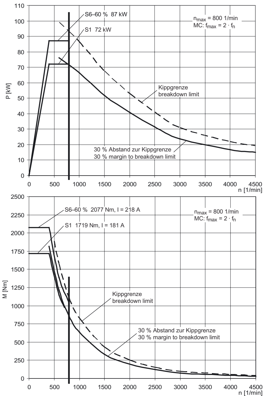
Figure 3-72 MASTERDRIVES MC, 1PL6228-□□B□□
