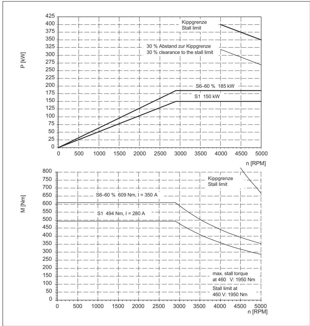
Figure 3-55 MASTERDRIVES VC, 1PL6186-□□L□□
