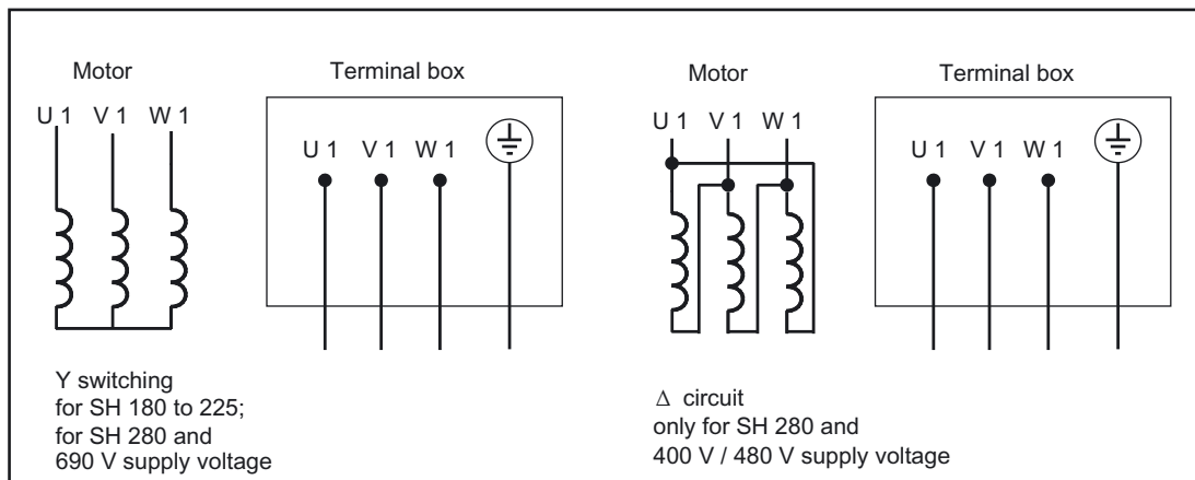
Figure 2-2 Circuit diagram
