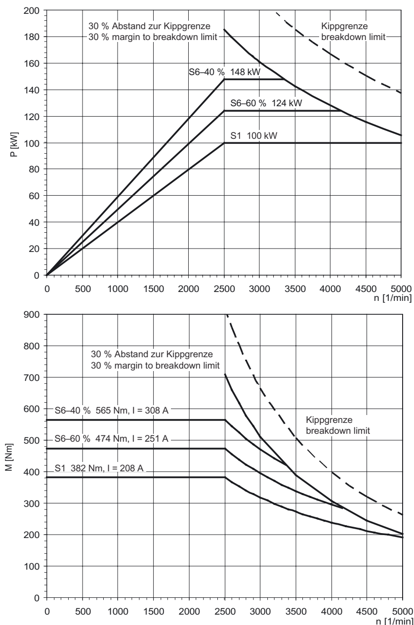
Figure 3-83 MASTERDRIVES MC, 1PL6184-□□L□□
