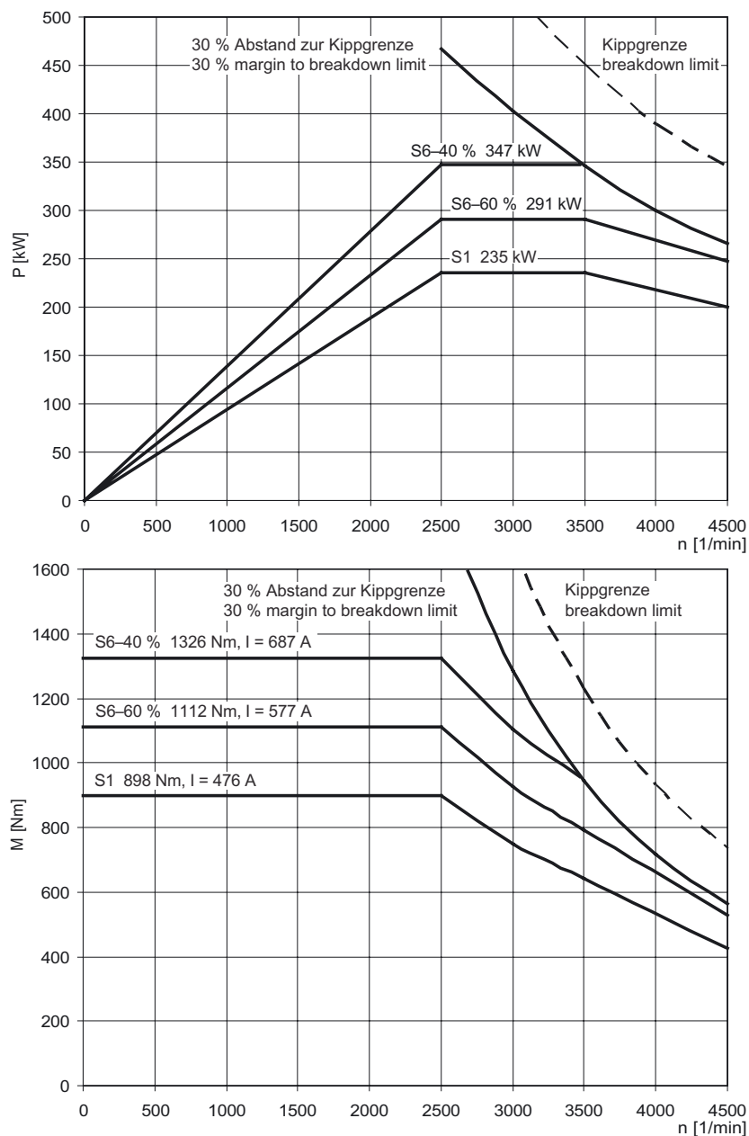
Figure 3-86 MASTERDRIVES MC, 1PL6226-□□L□□
