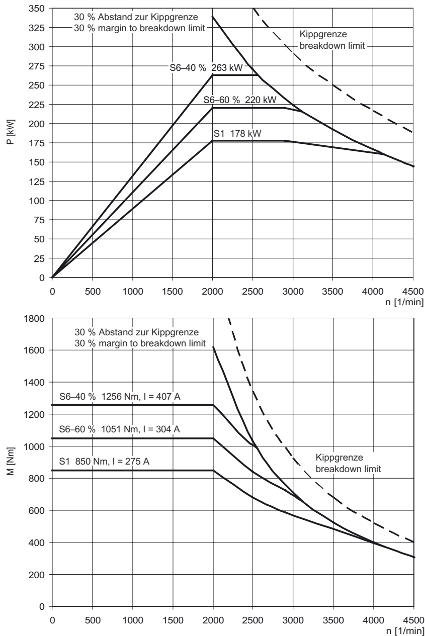
Figure 3-48 MASTERDRIVES VC, 1PL6224-□□F□□
