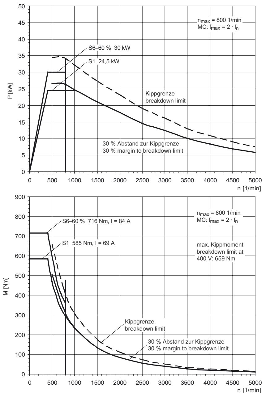
Figure 3-88 MASTERDRIVES VC, 1PL6184-□□B□□
