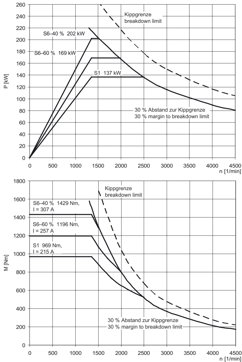
Figure 3-40 MASTERDRIVES VC, 1PL6224-□□D□□
