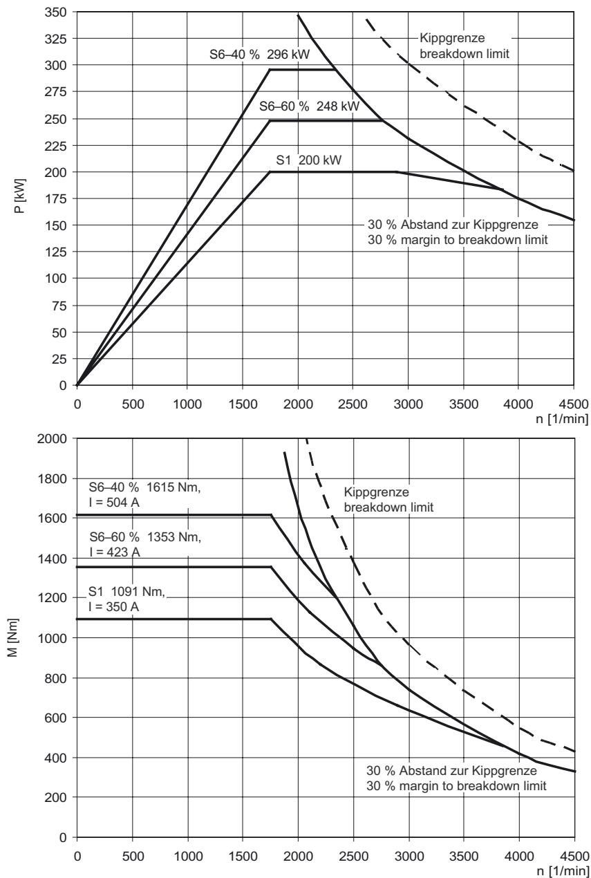
Figure 3-20 MASTERDRIVES VC, 1PL6226-□□F□□
