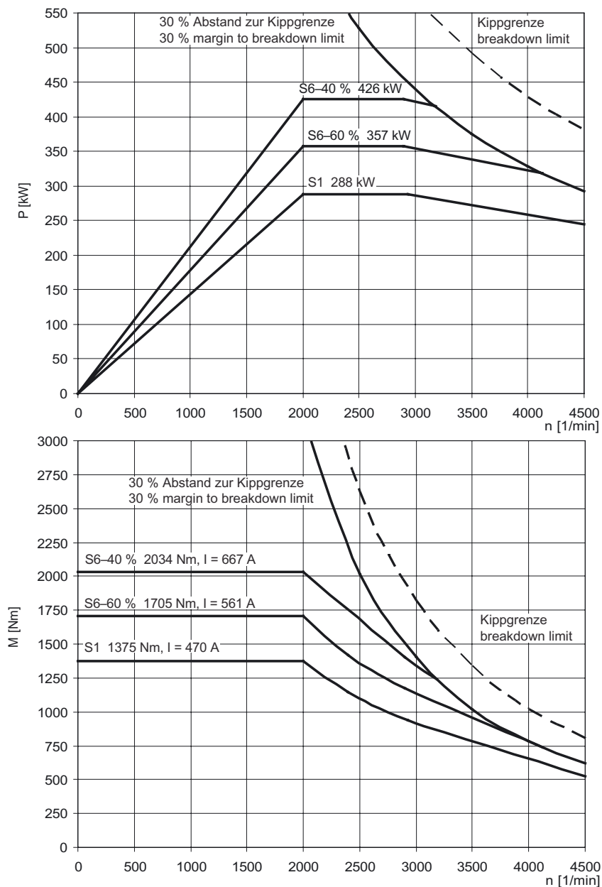
Figure 3-50 MASTERDRIVES VC, 1PL6228-□□F□□
