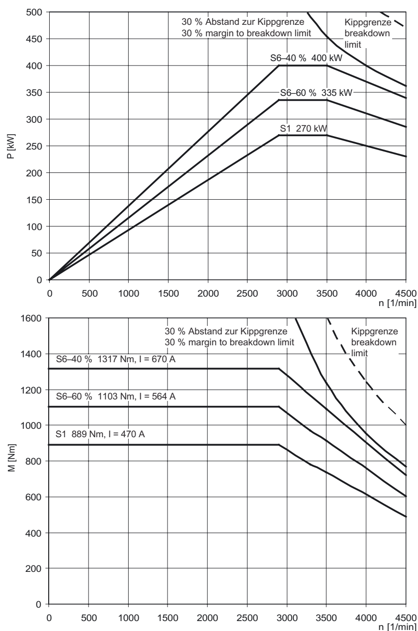
Figure 3-57 MASTERDRIVES VC, 1PL6226-□□L□□
