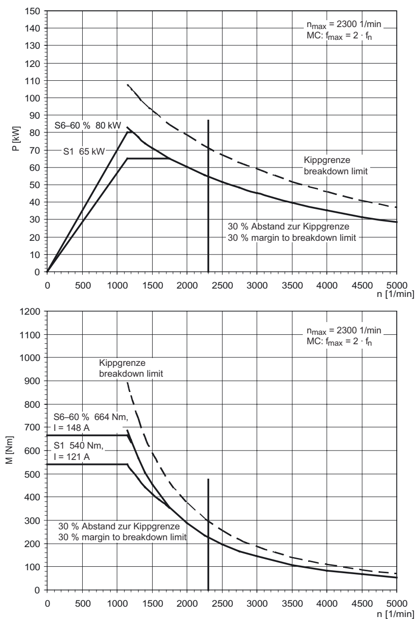
Figure 3-93 MASTERDRIVES MC, 1PL6184-□□D□□
