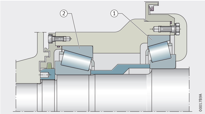
Figure 1 Axlebox bearing arrangement
