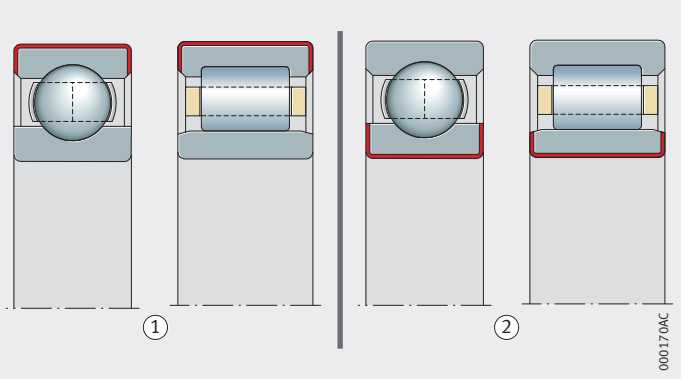
Figure 12 Types of coatings
