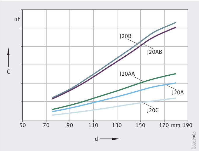
Figure 11 Relationship between electrical capacitance and coating used
