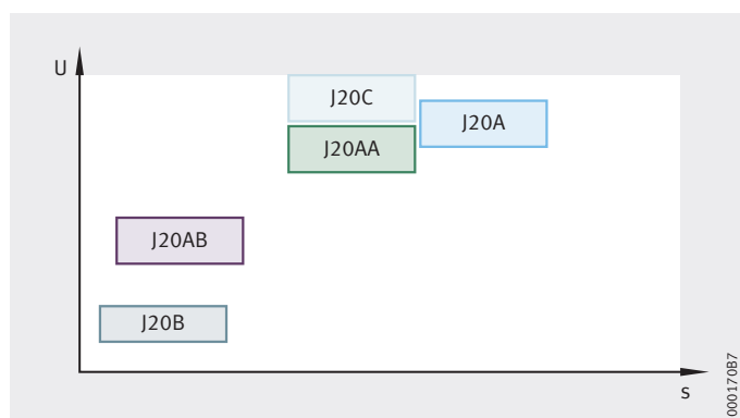
U = puncture voltage s = coating thickness Figure 8 Overview of coatings
