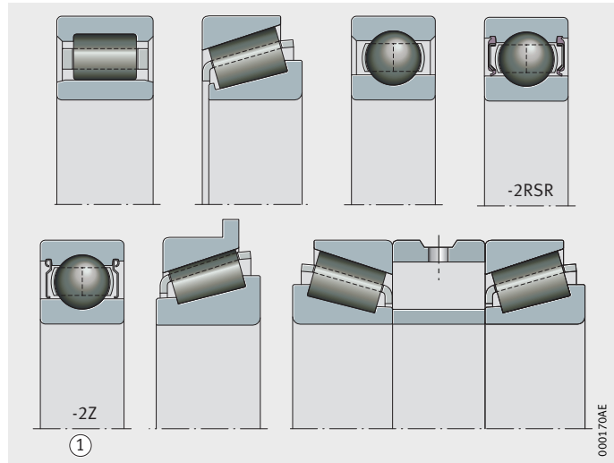
Figure 13 Bearing designs
