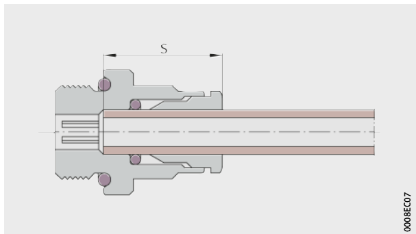
Figure 13 Insertion depth
