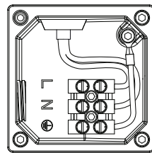
VPC-B215xx Motors
