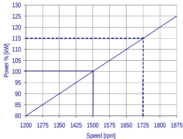
SPEED/POWER DIAGRAM
