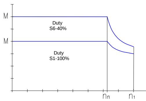
TORQUE DIAGRAM
