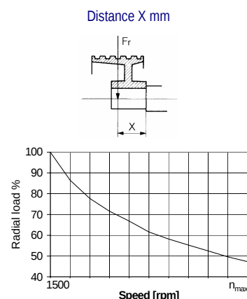
Radial load diagram
