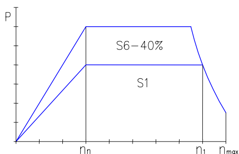
POWER DIAGRAM
