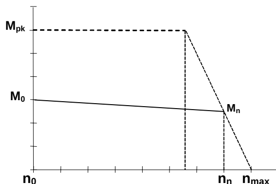
TORQUE DIAGRAM
