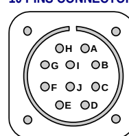
10 PINS CONNECTOR
