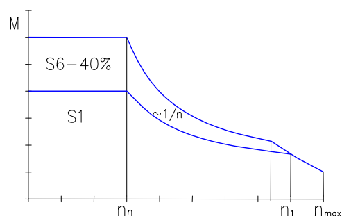
TORQUE DIAGRAM
