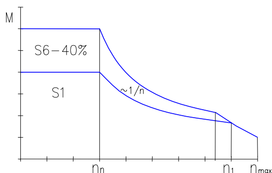
TORQUE DIAGRAM
