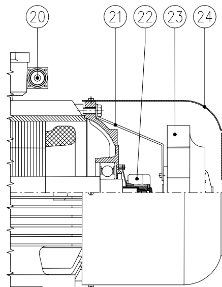
SERVO-VENTILATED
