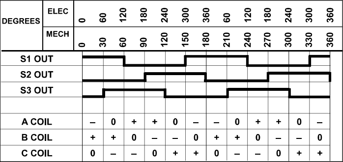
Timing Diagram (4 Pole) CCW Rotation
