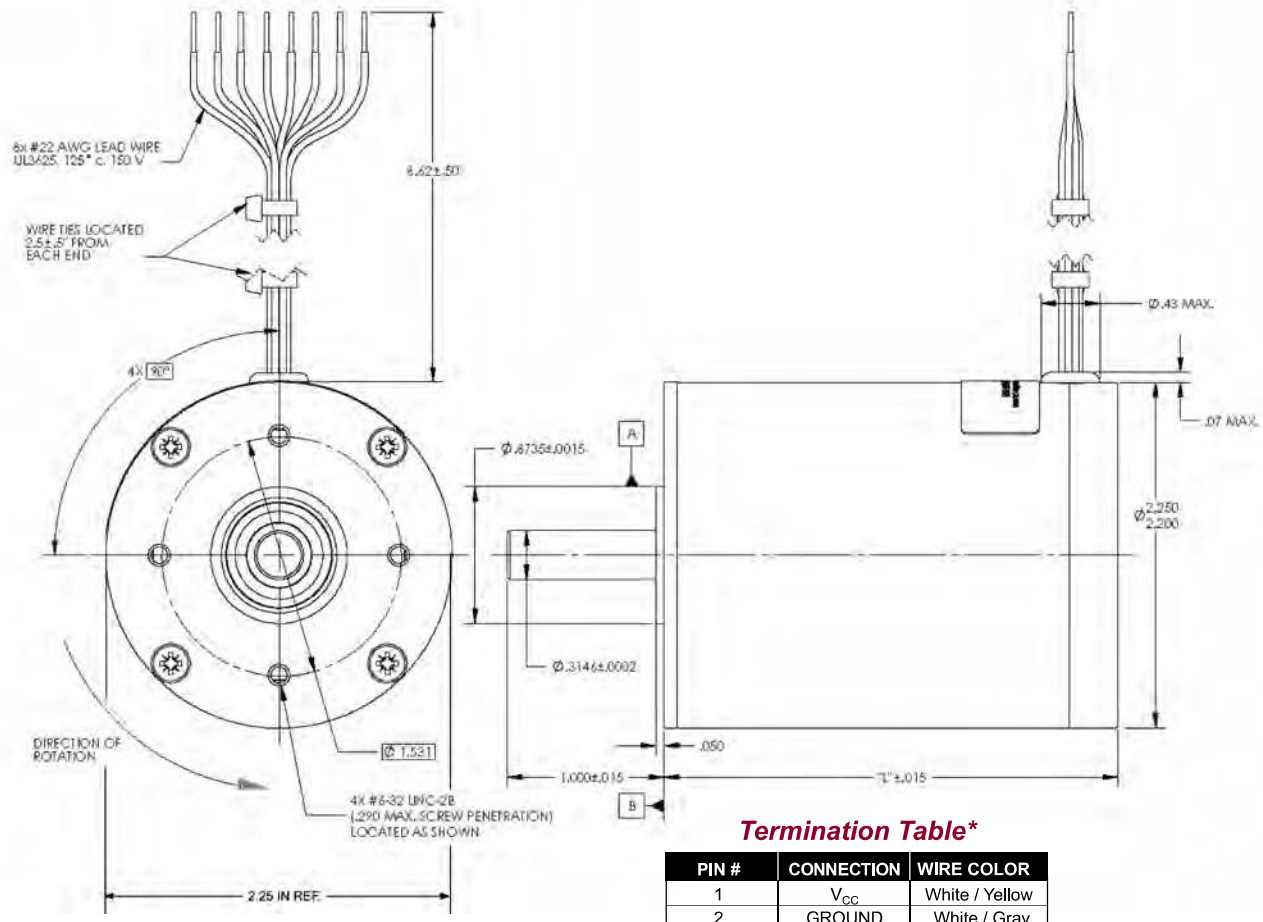
Typical Outline Drawing - BN23
