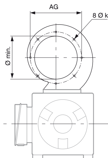
Configuration for LSK 3554
