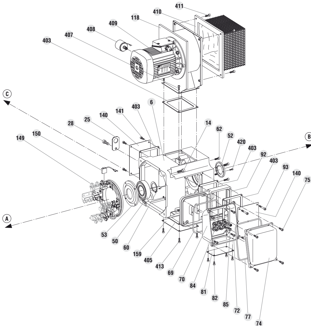
LSK motor models 1124 to 1604
