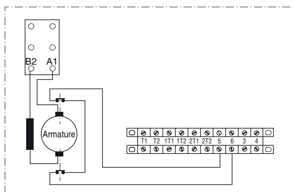
Diagram 1. - Connection of the brush wear limit probe For LSK 1124 to 2254 (for LSK 2504 to 3554 : diagram on request)
