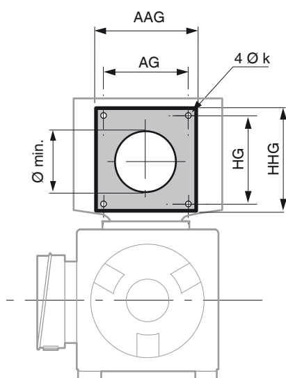
Configuration for LSK 1124 to 1804
