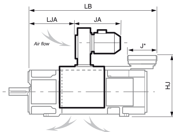
Dimensions with forced cooling unit blowing on the body (IC 416)
