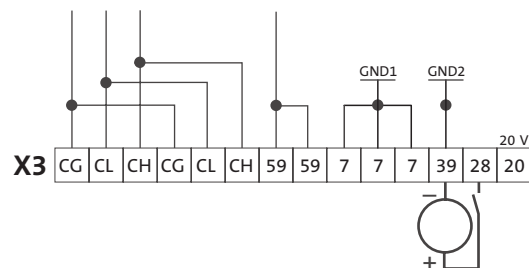
Supply for function module and controller inhibit (CINH) via external voltage source
