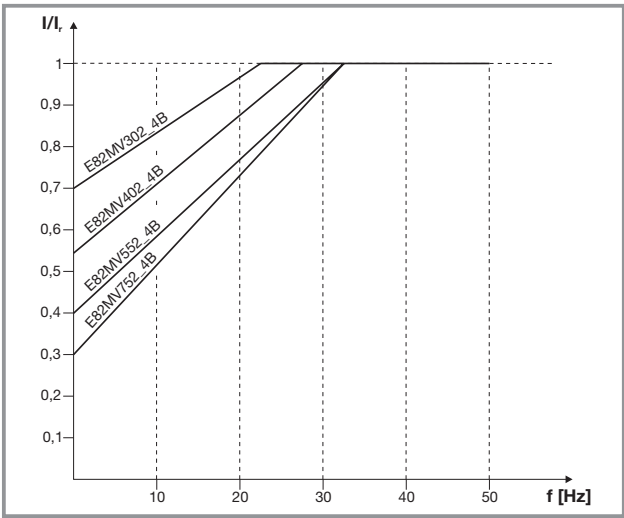
Figure 1: Derating of rated output current in continuous operation at 40°C ambient temperature and switching frequency 4 kHz or at 35°C and 8 kHz.
