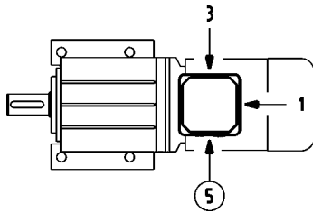
Terminal box in position 2
