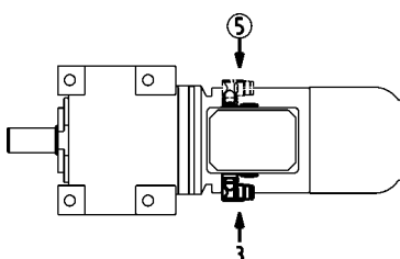
Terminal box in position 4
