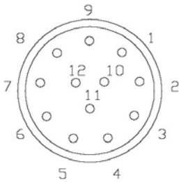
Signal connector
