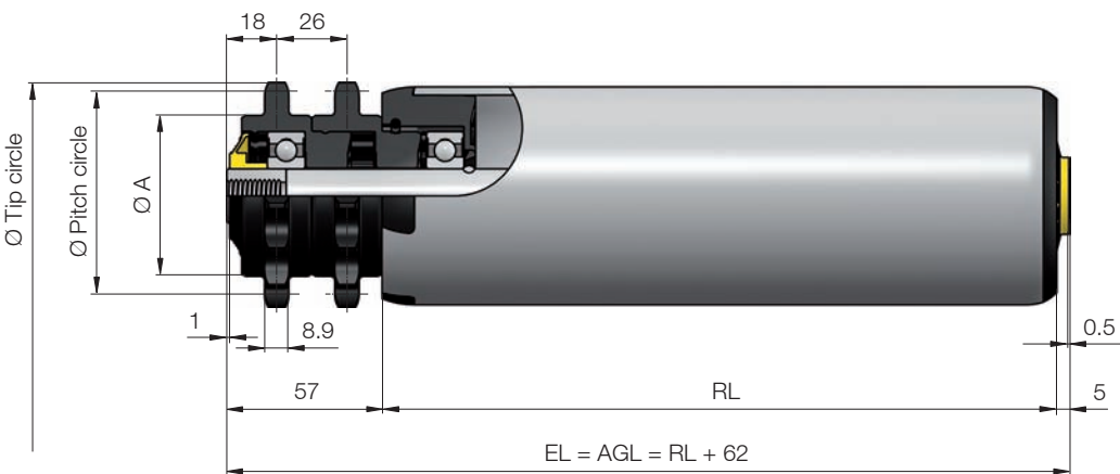
Dimensions for 2 polymer sprockets 5/8", without flange
