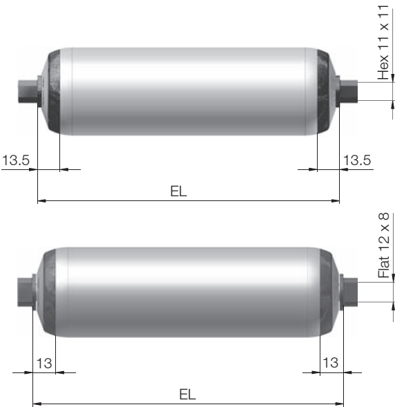
Shaft adapter
