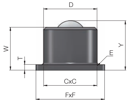
Dimensions with base flange
