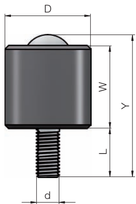
Dimensions with threaded pin
