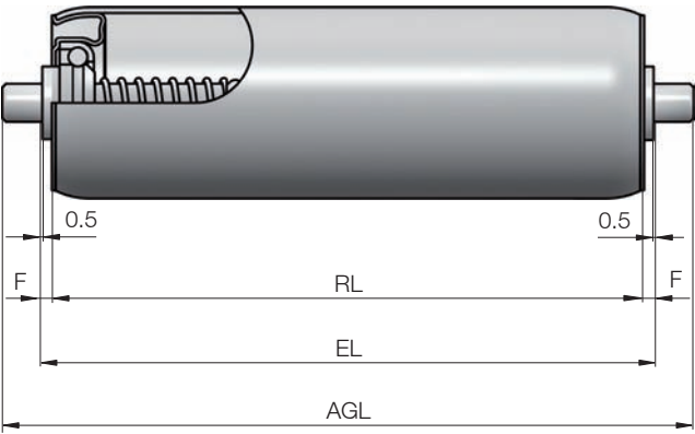
Dimensions for spring-loaded shaft
