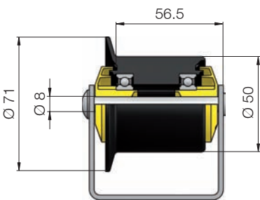
Fig.: Dimensions with polymer conveyor roller with flange
