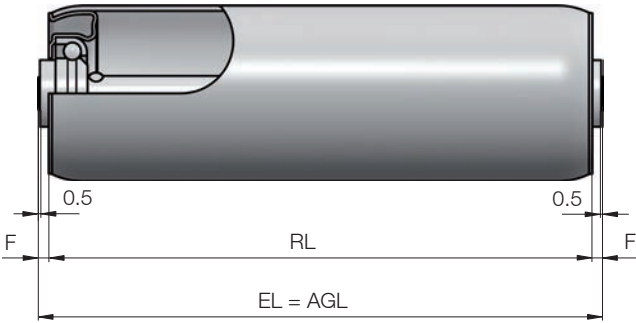
Dimensions for female threaded shaft M8 x 15
