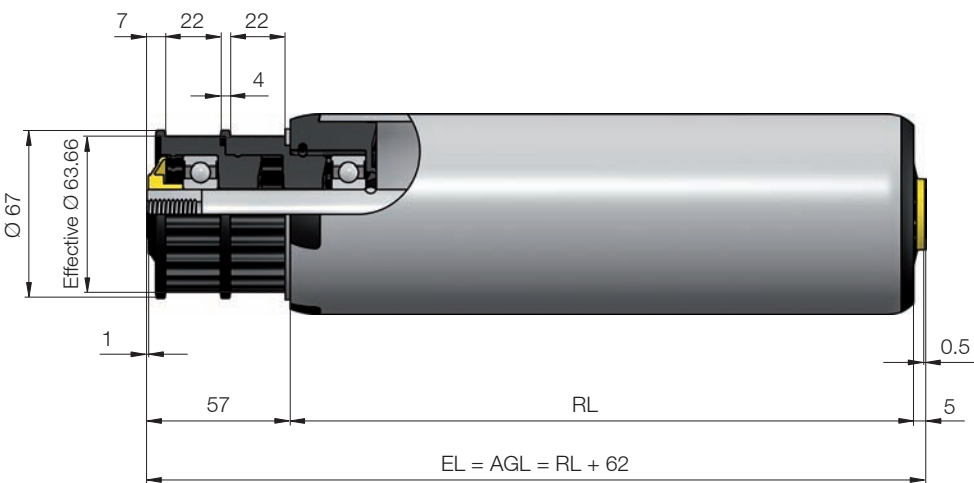
Dimensions for flange
