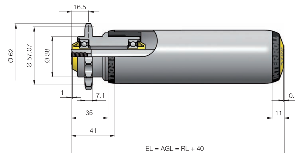
Dimensions for 2 steel sprockets 1/2", Z = 14
