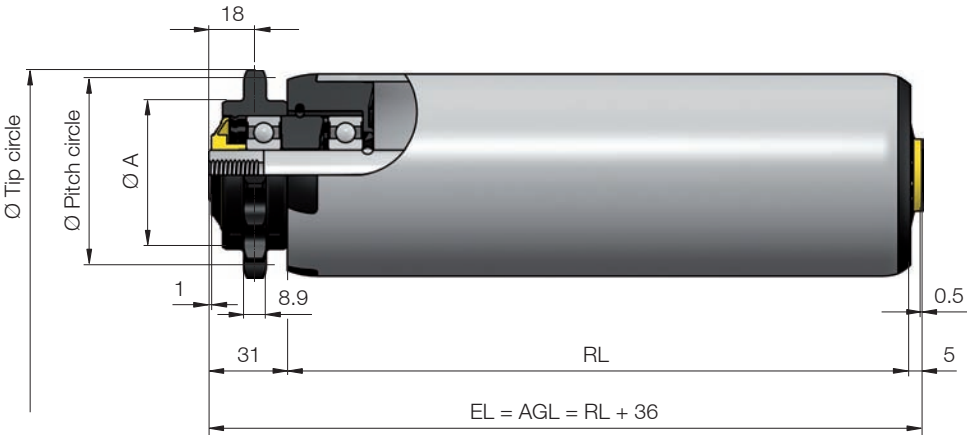
Dimensions for polymer sprocket 5/8", without flange
