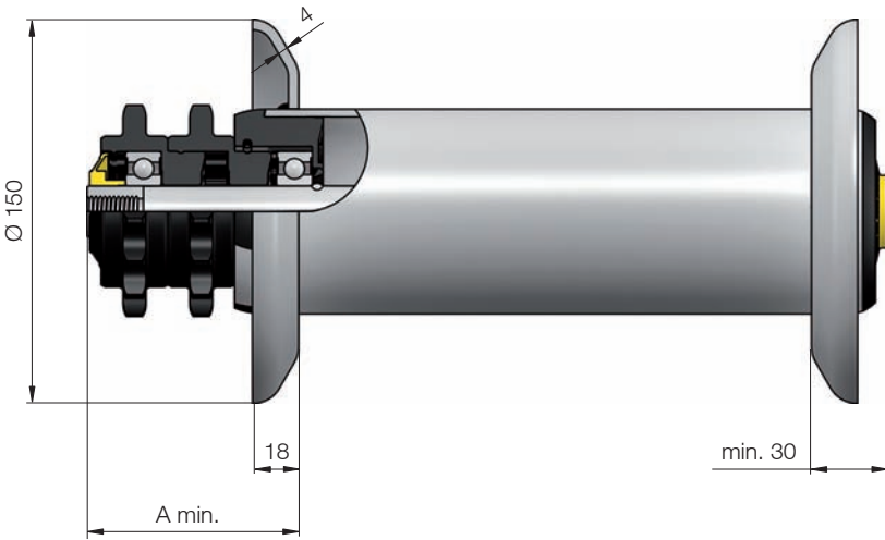
Dimensions for flange
