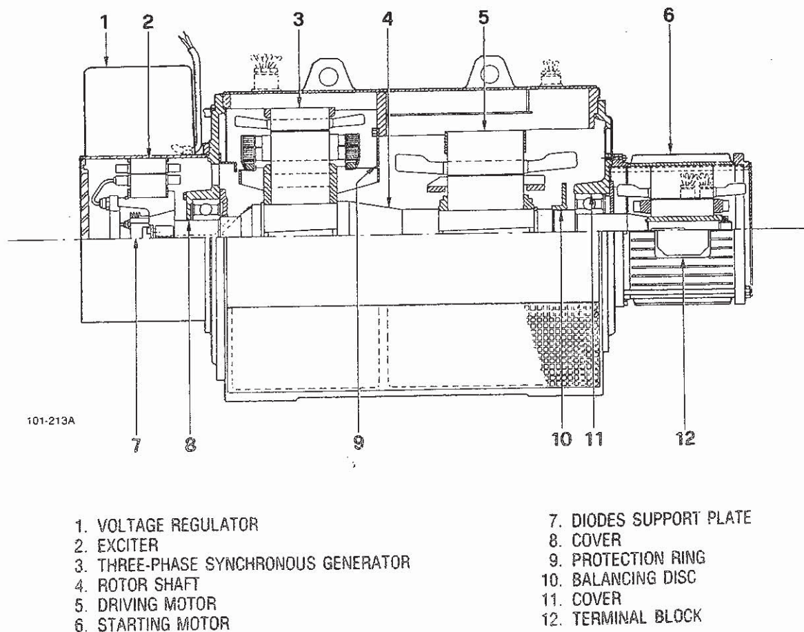
Figure 1-2. Frequency Converter - Main Components
