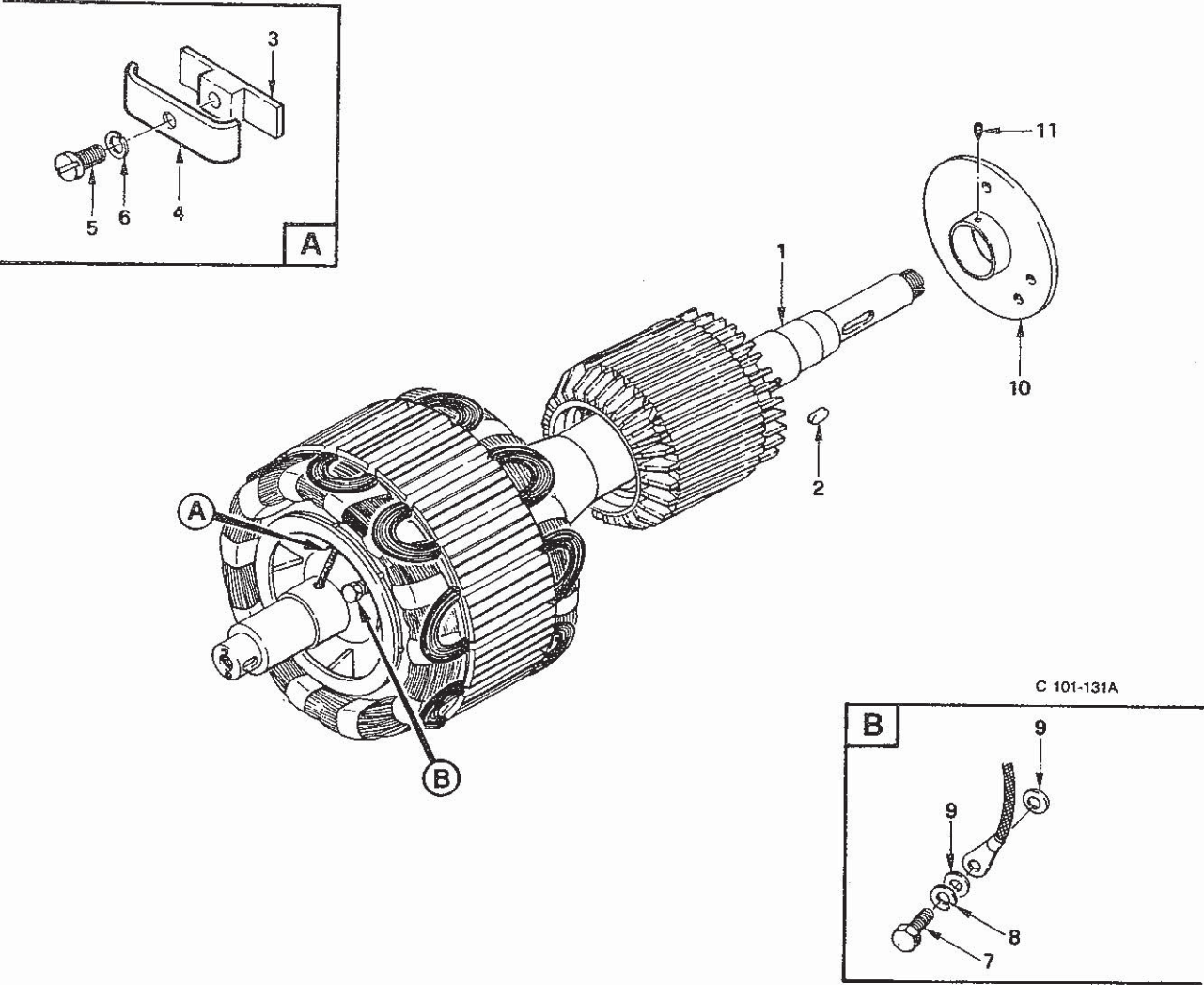
Figure 10-4. Rotor Assembly
