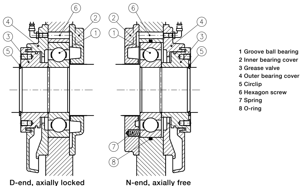
Figure: Standard bearing construction for horizontally mounted motors, frame sizes 355-500.
