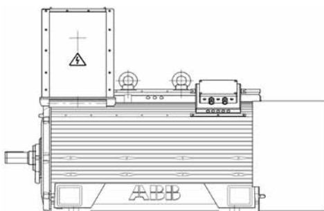
Code I: IM B3 Code II: IM 1001 Standard floor mounting, feet facing downwards (Horizontal foot mounted)
