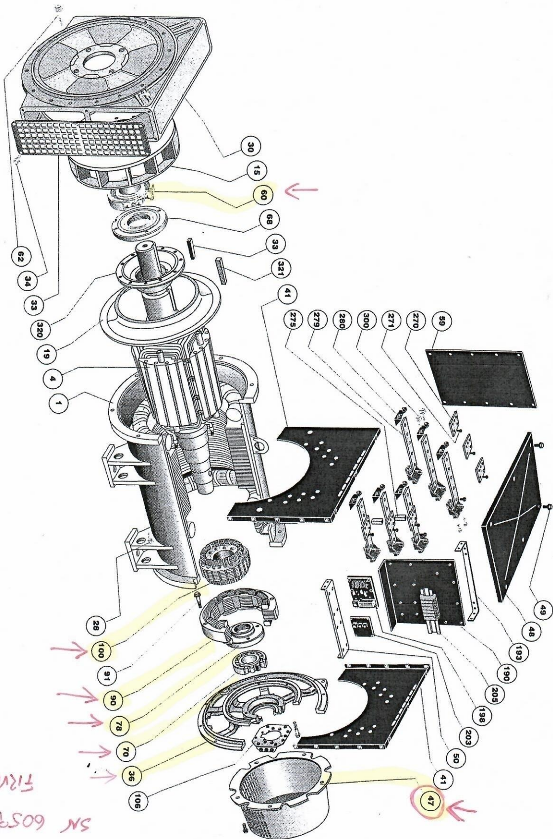
5.3.5 - Exploded view : two-bearing LSA 51.2
