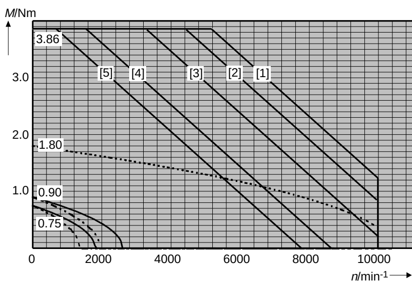
Fig 4.5: Torque-speed characteristics curves - MDD 025
