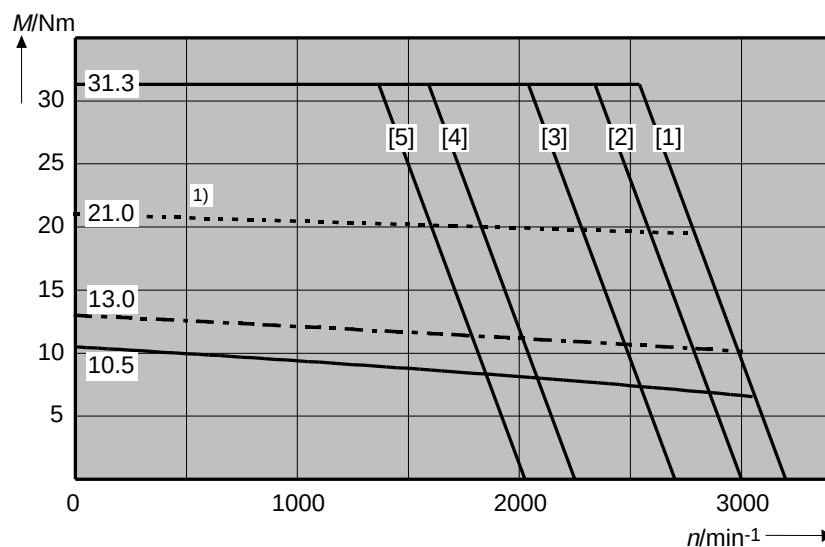
Fig 10.4: Torque-speed characteristics curve MDD 112
