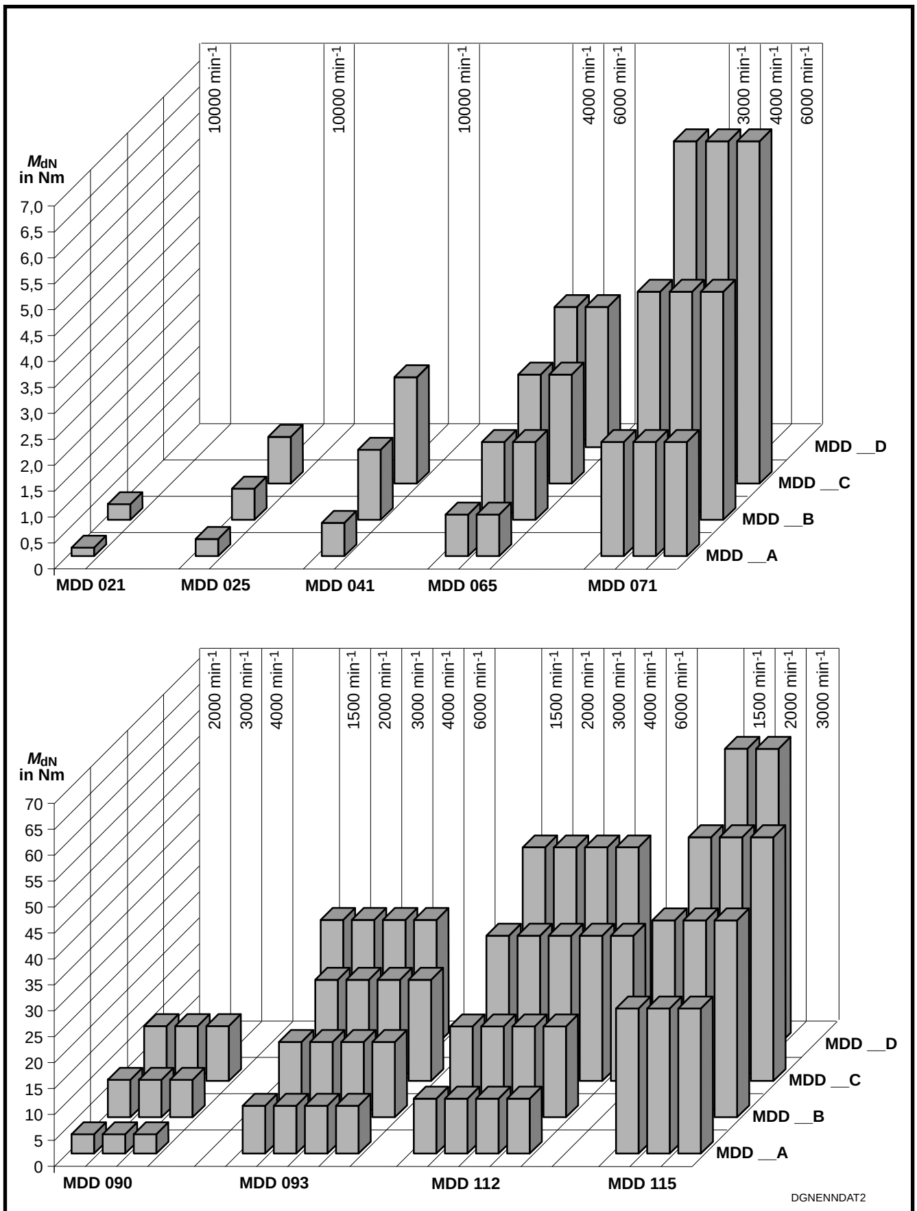
Fig. 1.1: Power levels
