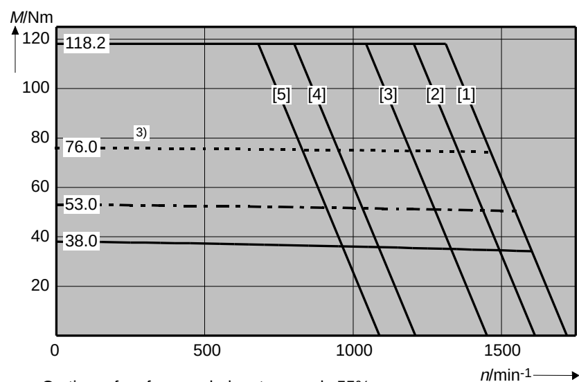
Fig 11.5: Torque-speed characteristics curve - MDD 115
