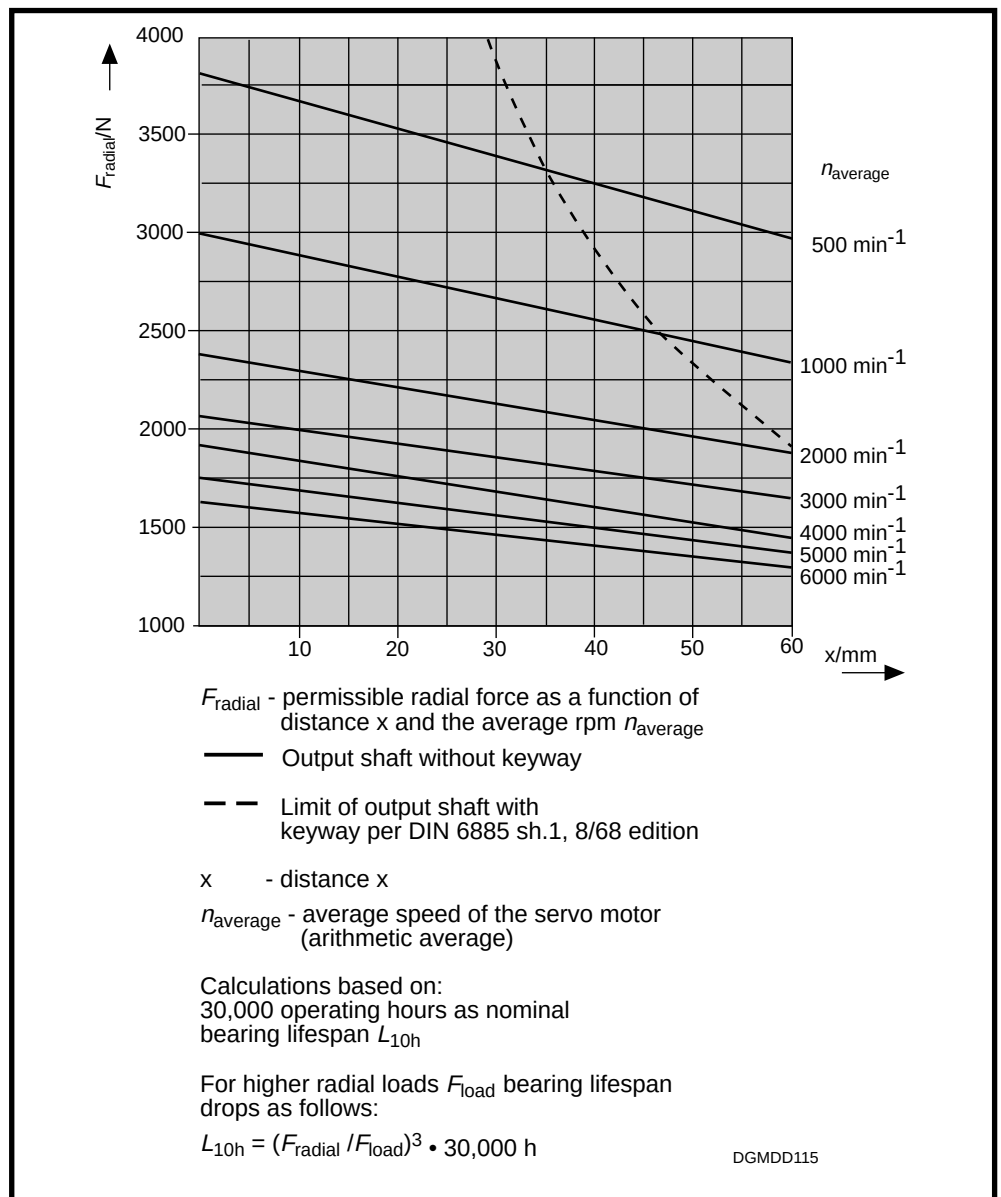
Fig 11.10: Permissible radial force
