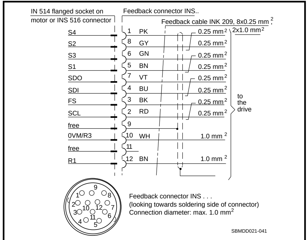
Fig 13.1: Terminal diagram for the motors with "resolver feedback"
