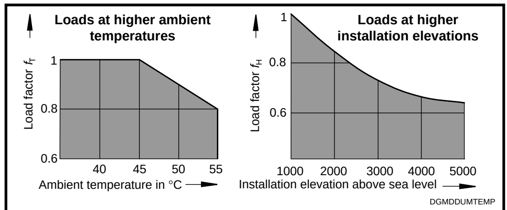
Fig. 2.1: Load capabilities at higher ambient temperatures and higher installation elevations
