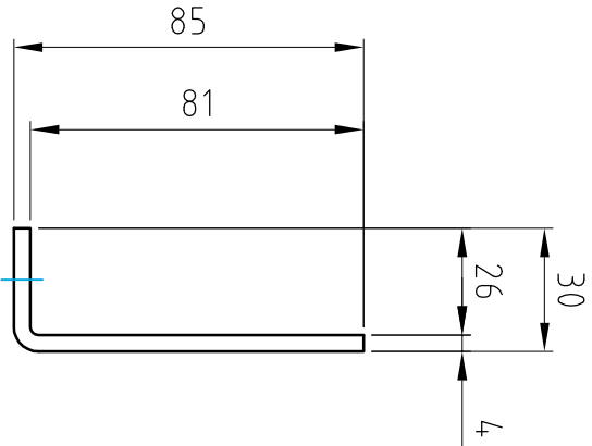
VISTA A (1:2)
