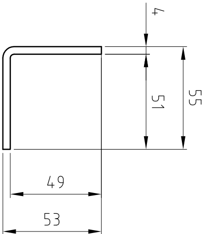
VISTA A (1:2)
