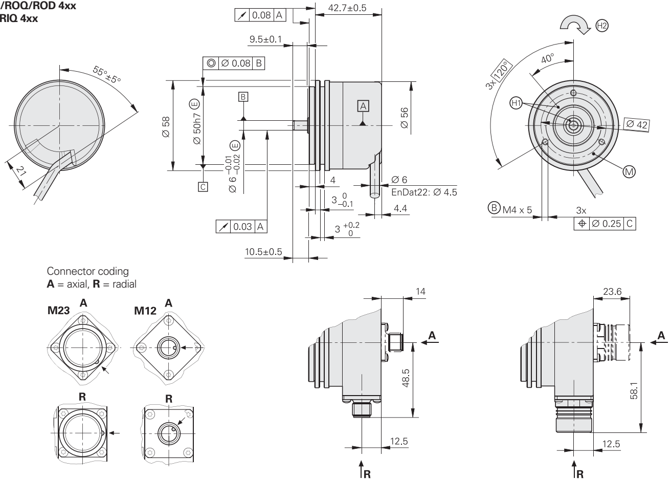
ROC 413/ROQ 425 with PROFIBUS DP/PROFINET IO
