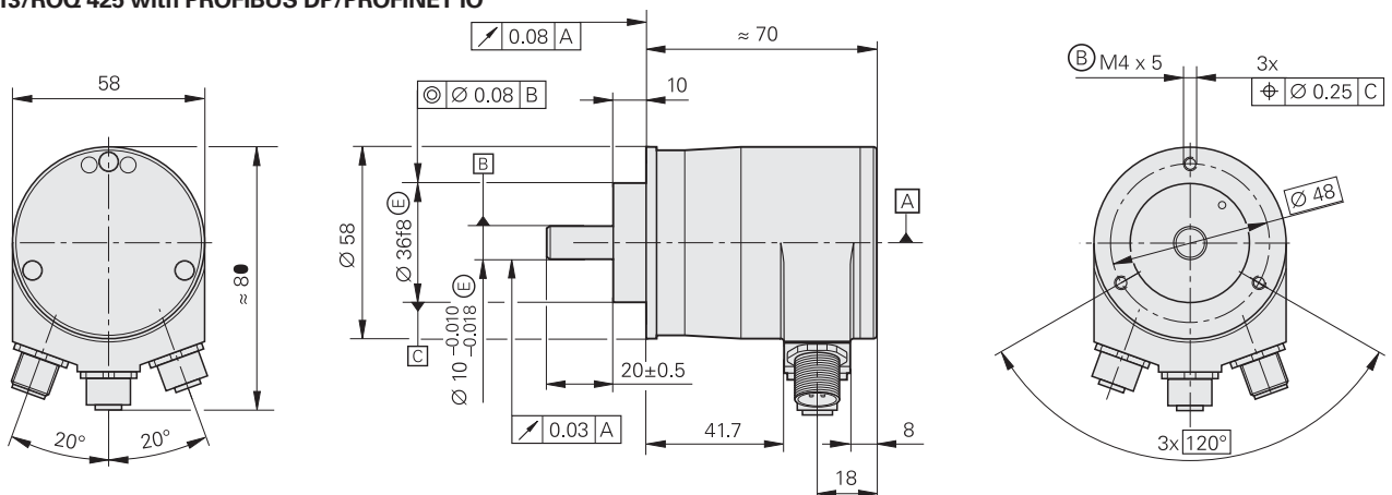
ROC 413/ROQ 425 with PROFIBUS DP/PROFINET IO
