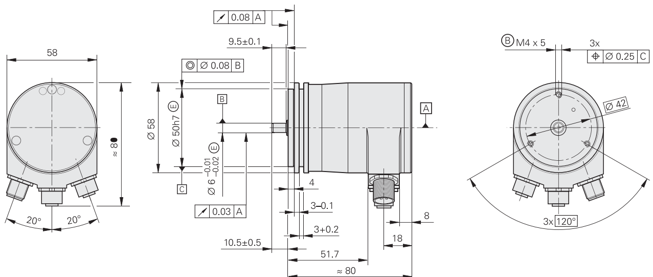
ROC 413/ROQ 425 with PROFIBUS DP/PROFINET IO
