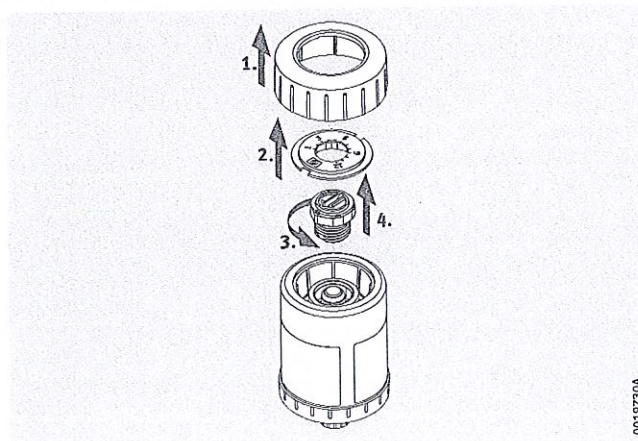
Figure 24 Detach drive unit
