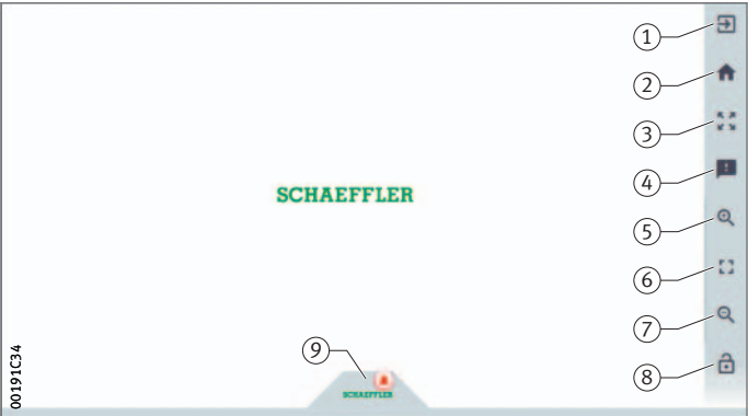
Figure 57 Start page
