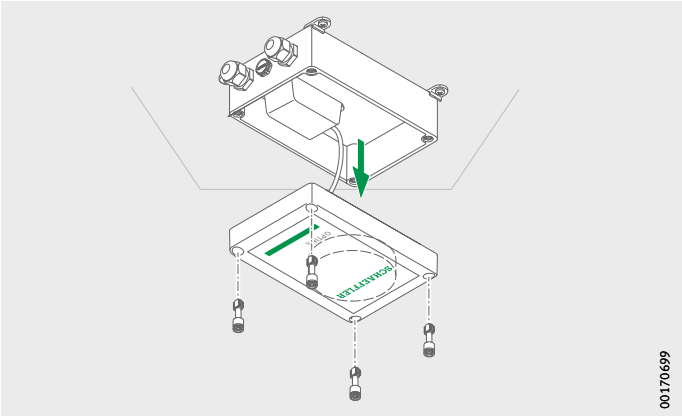
Figure 14 Open cover
