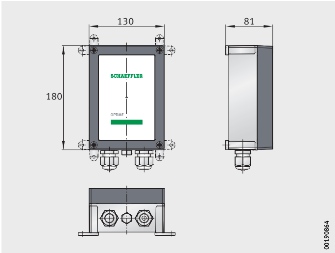
Figure 65 Gateway dimensions
