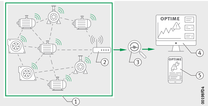
① Mesh network ② OPTIME gateway ③ Schaeffler IoT Hub ④ OPTIME dashboard ⑤ OPTIME app Figure 7 Communication between OPTIME system components
