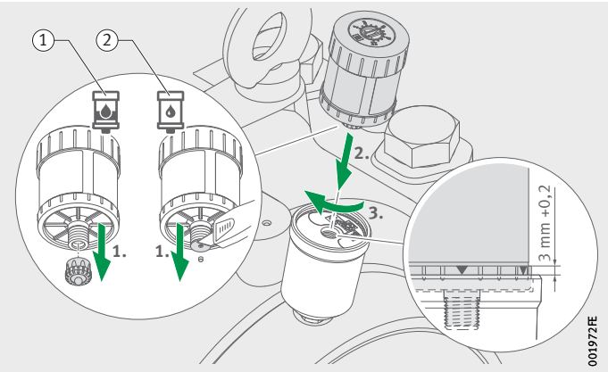
Figure 22 Screw-mount cartridge CONCEPT1
