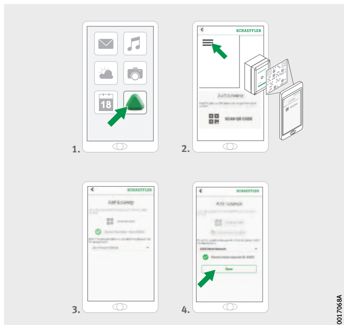
Figure 11 Add gateway
