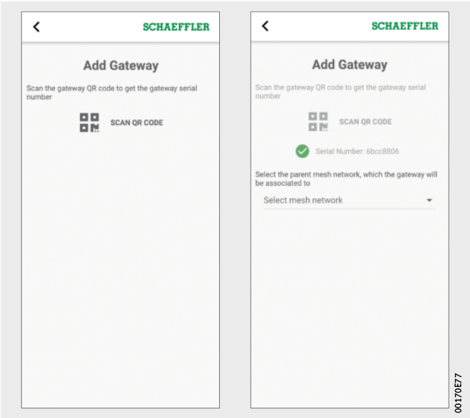
Figure 52 Add gateway
