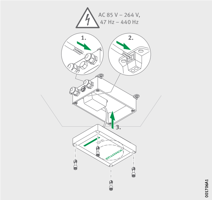
Figure 15 Complete the electrical connections to the gateway
