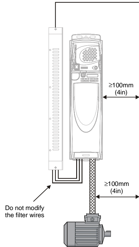
Figure 4: Input wiring spacing
