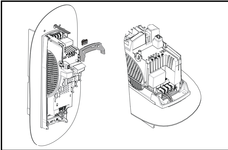
Figure 1-6 Unidrive SP size 1 DC connections
