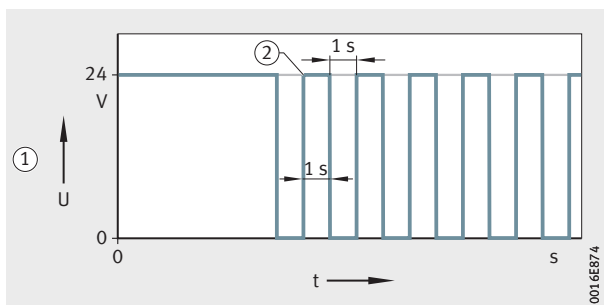
Figure 17 Output signal for empty level
