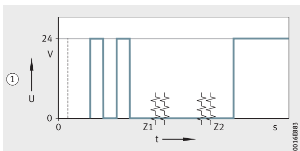
Figure 18 Output signal when changing the cartridge
