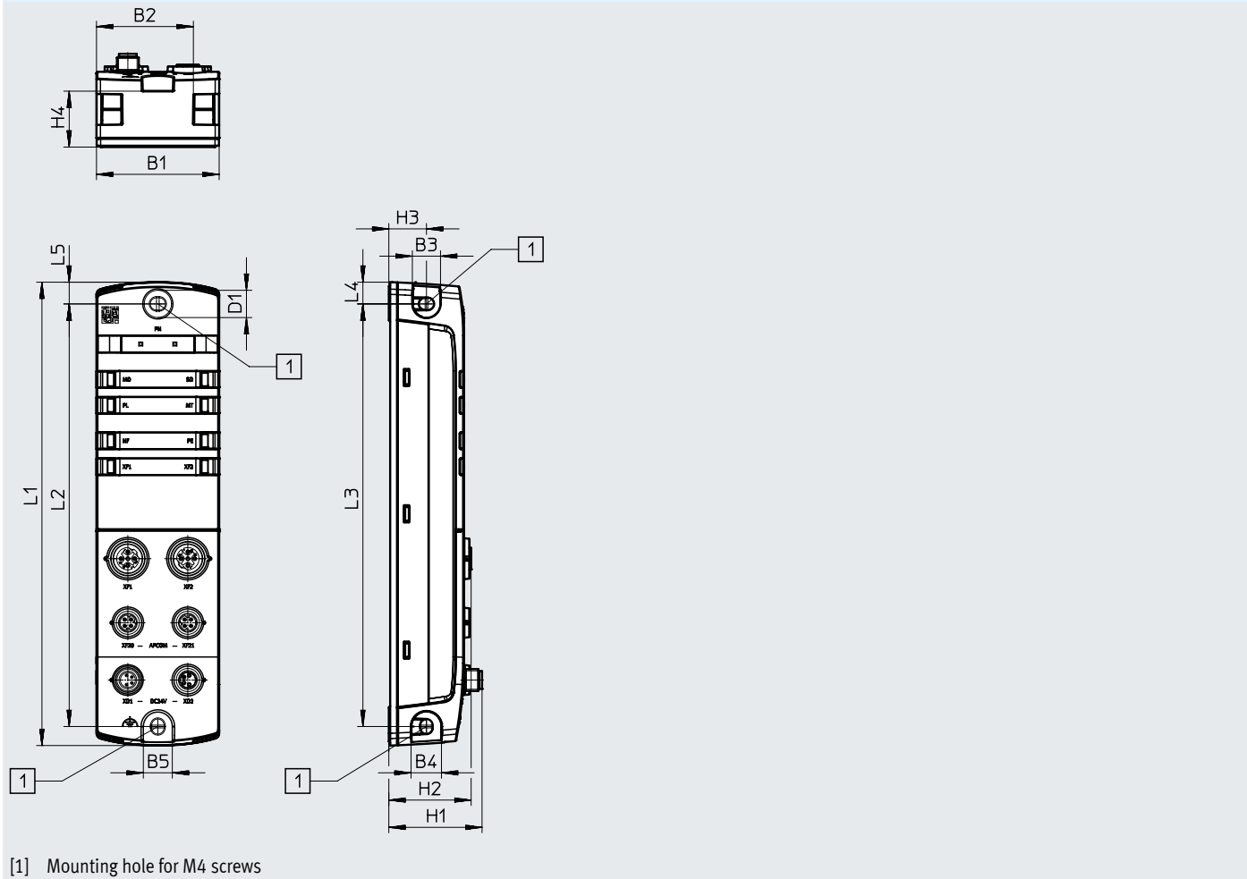
[1] Mounting hole for M4 screws
