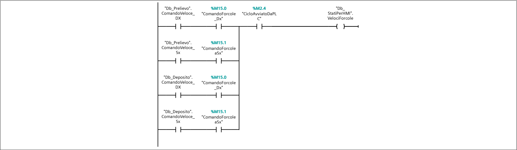
Segmento 9: set point
