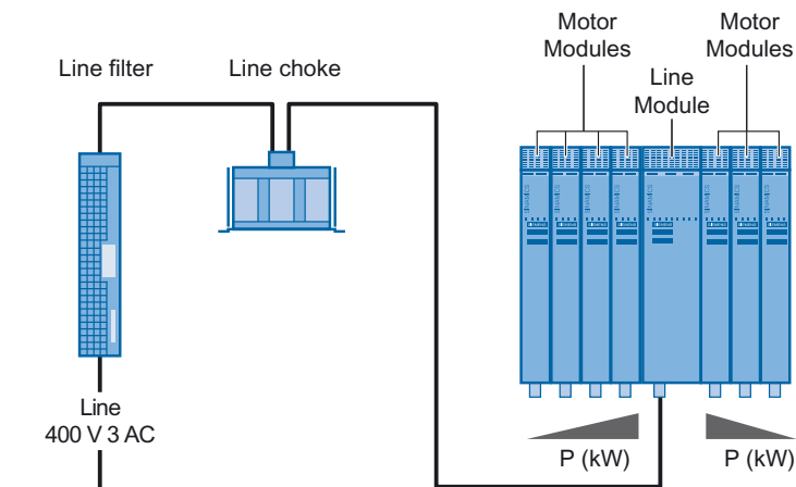
Figure 2-5 Center infeed construction
