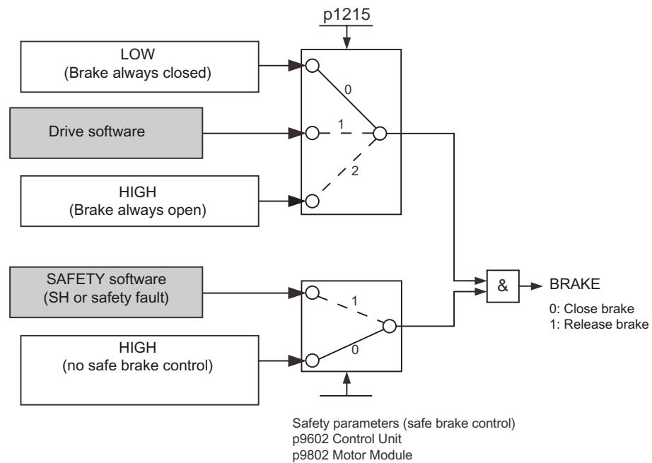
Figure 5-39 Operating modes of the safe brake control
