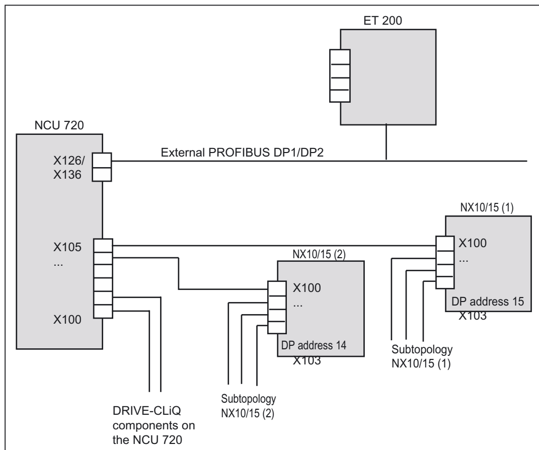
Figure 5-17 NX10/15 topology
