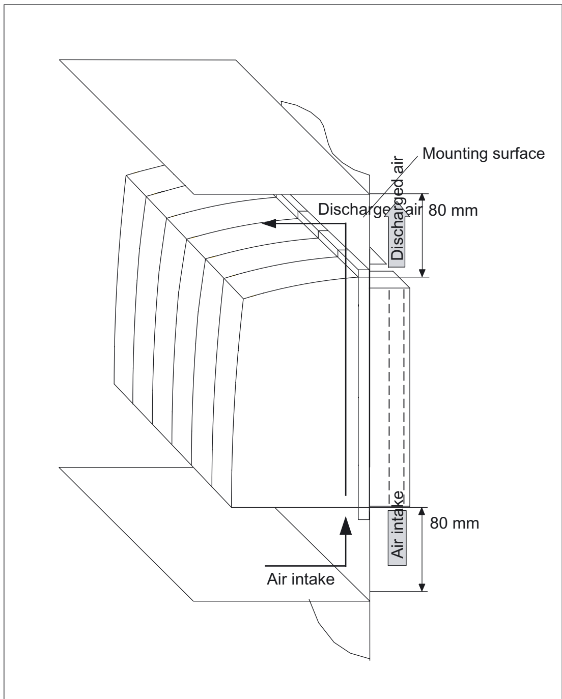
Figure 2-22 Clearances for booksize drive line-up with external air cooling
