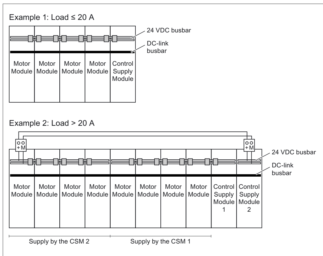
Figure 5-22 24 VDC division
