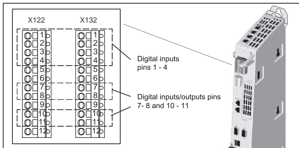
Figure 3-2 X122 and X132 interfaces for NCU 7x0
