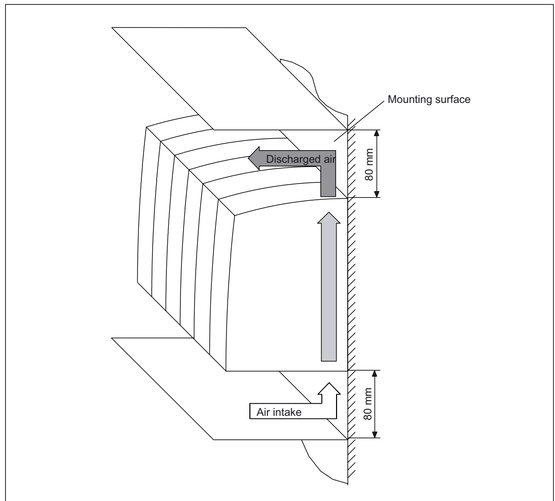
Figure 2-21 Clearances for booksize drive line-up with internal air cooling
