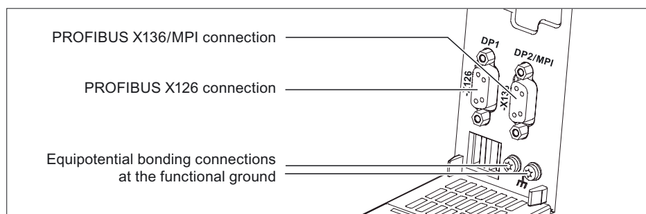
Figure 5-24 PROFIBUS and function ground connections
