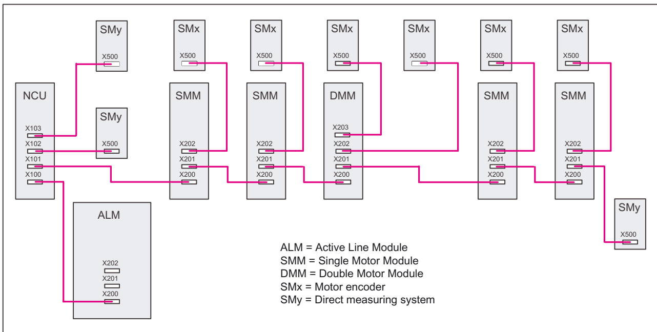
Figure 5-16 DRIVE-CLiQ wiring
