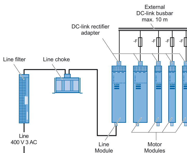
Figure 8-1 Distributed Installation
