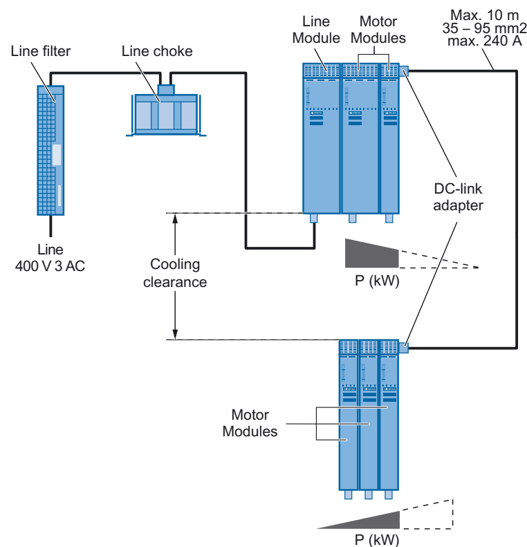
Figure 2-3 Two-row construction
