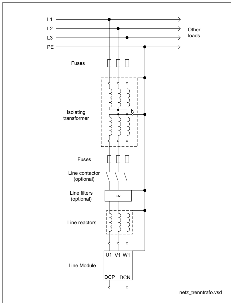
Figure 5-4 Isolating transformer
