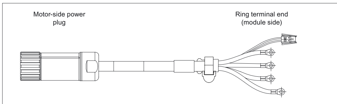
Figure 5-28 Motor Module - motor connection for Motor Modules > 30 A
