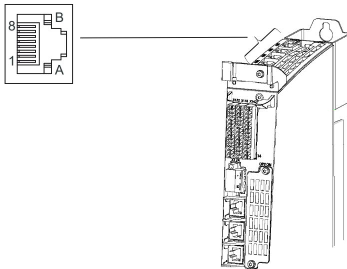
Figure 7-4 DRIVE-CLiQ interfaces
