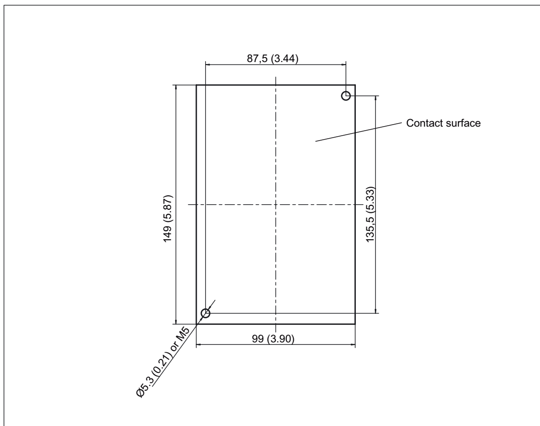
Figure 3-54 DME20 installation
