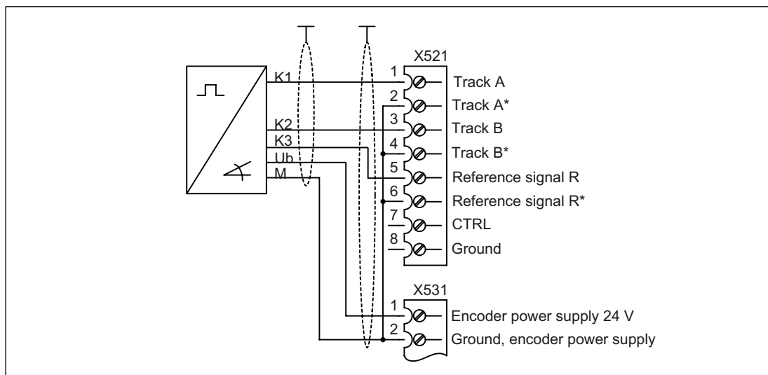
Figure 4-16 Connection example 2: HTL encoder, unipolar, with reference signal 1)
