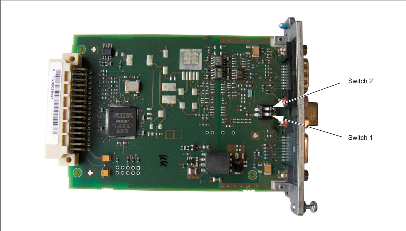
Figure 3-5 Switch 2/1
