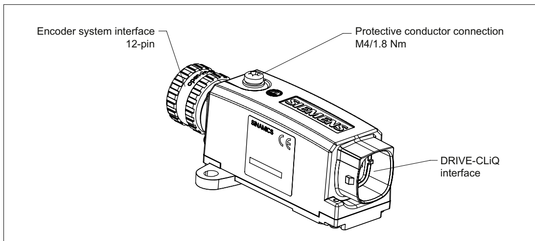
Figure 4-24 Interface description SME20
