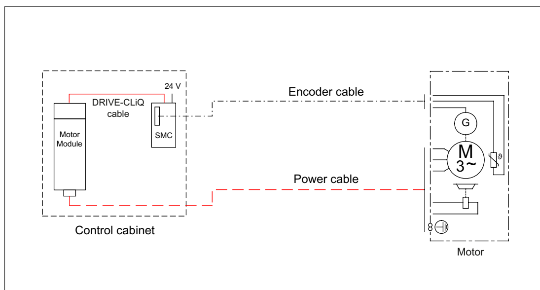
Figure 4-5 Connection of an encoder system via a Sensor Module Cabinet-Mounted (SMC) for a motor without a DRIVE-CLiQ interface
