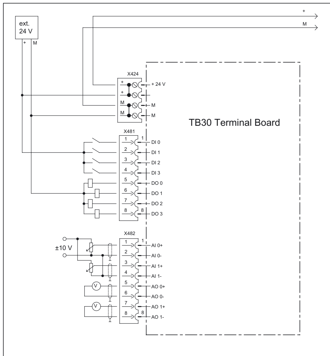
Figure 3-12 Example connection of TB30
