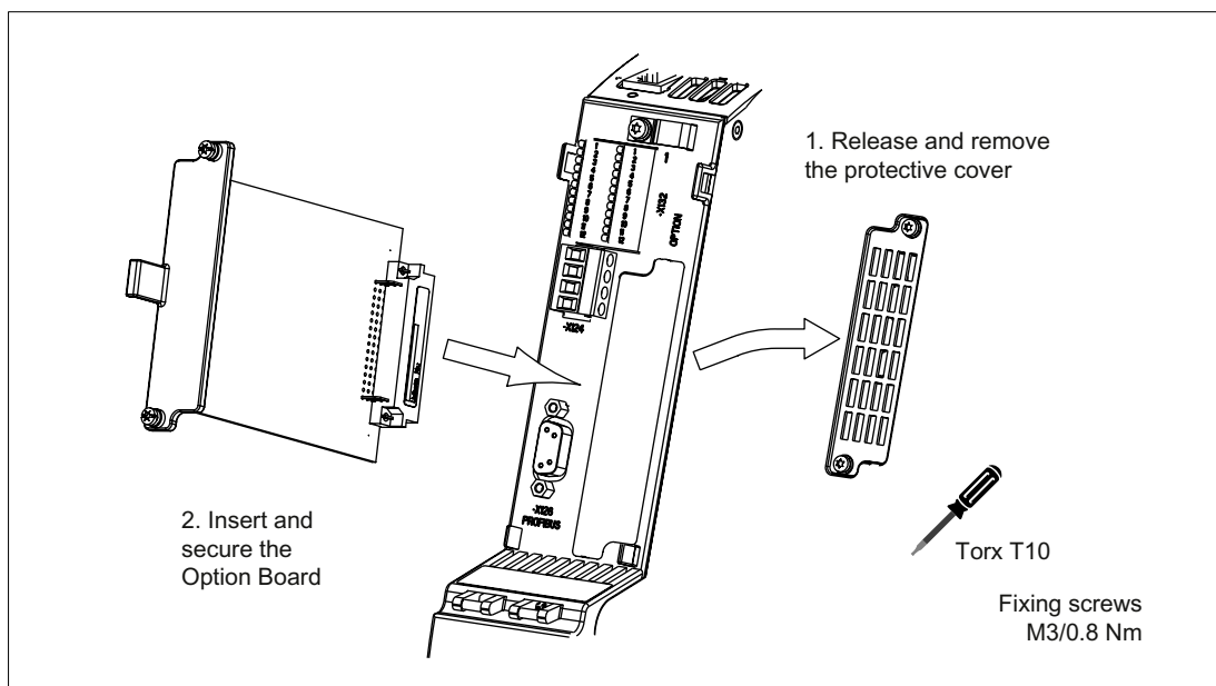
Figure 3-7 Installing an Option Board in a CU320
