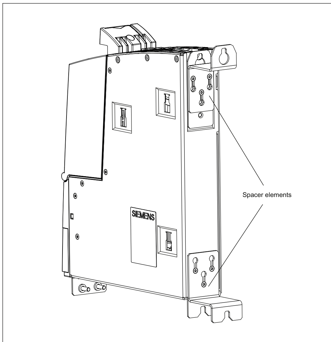
Figure 2-18 Installing the CU320-2 DP on a mounting surface using spacer elements
