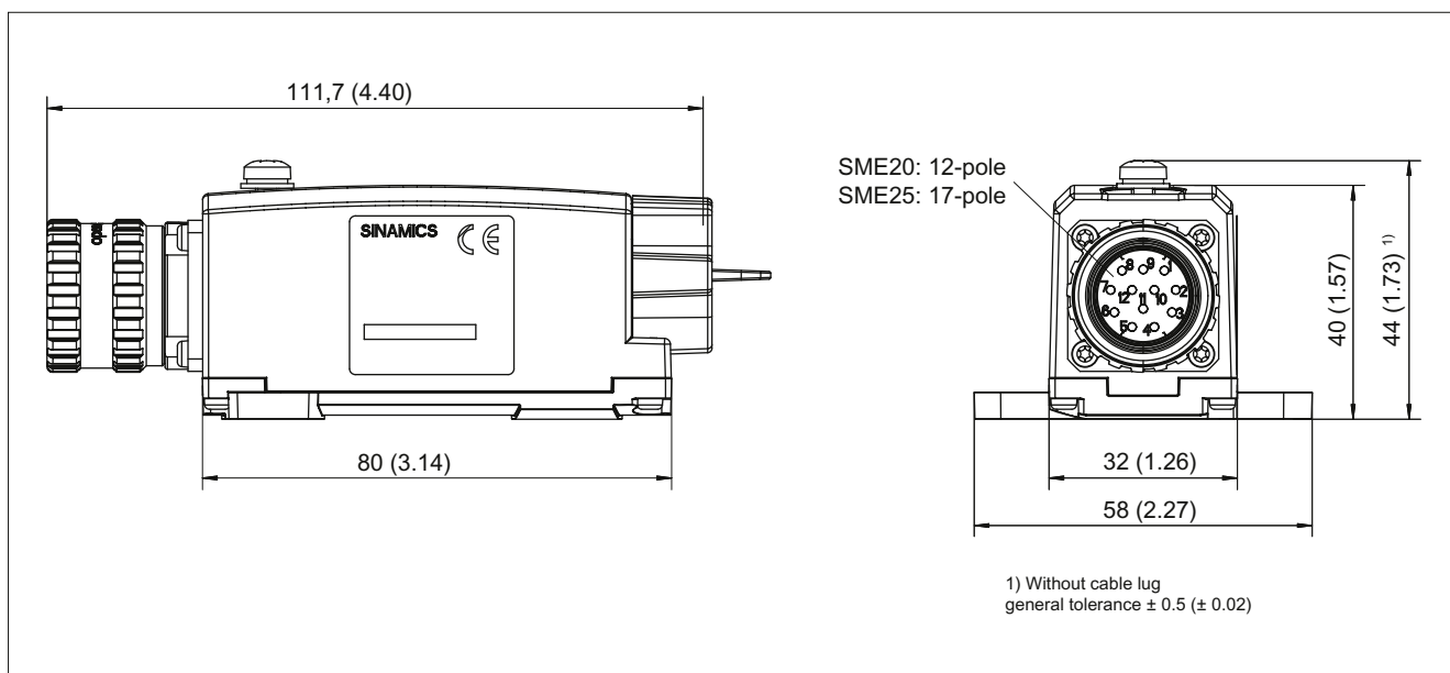
Figure 4-26 Dimension drawing of Sensor Module External SME20, all data in mm and (inches), order number 6SL3055-0AA00-5EA3
