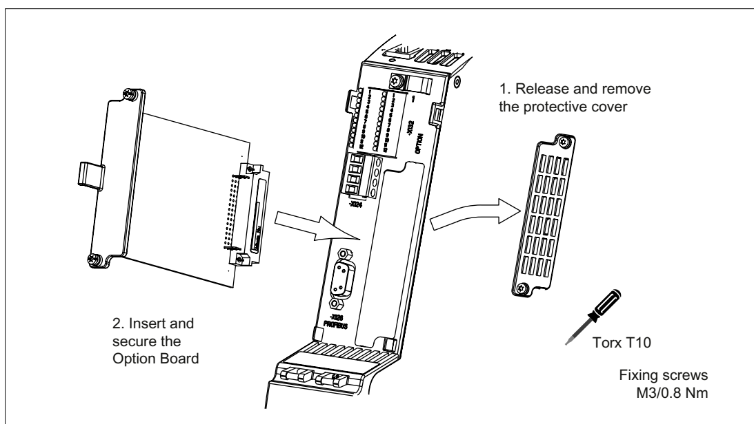
Figure 3-10 Installing the Option Board in a CU320
