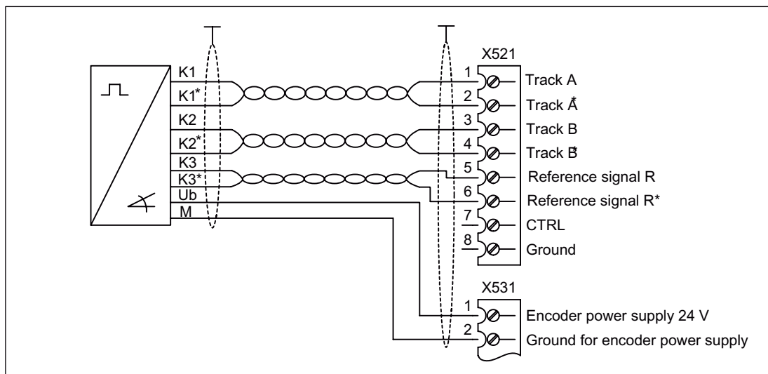
Figure 4-15 Connection example 1: HTL encoder, bipolar, with reference signal
