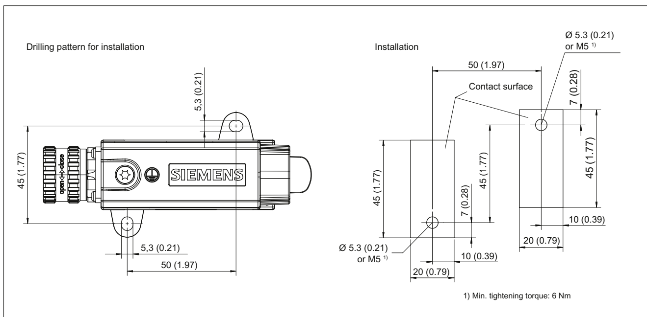
Figure 4-34 SME20/SME25 installation
