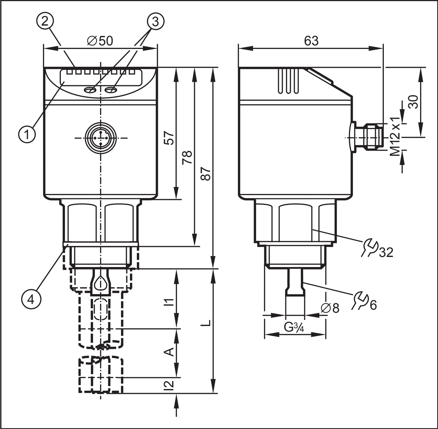
Dimensions in mm 1: display; 2: status LEDs; 3: programming buttons; 4: seal
