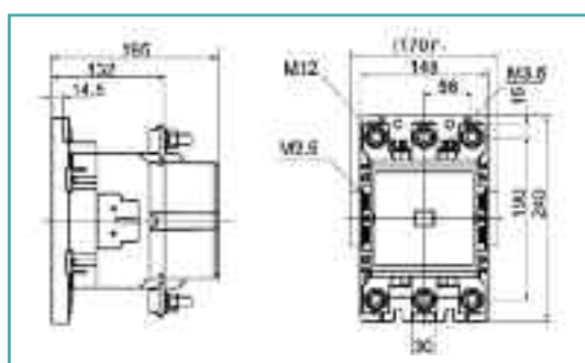
SC N14, N16 AC/DC
