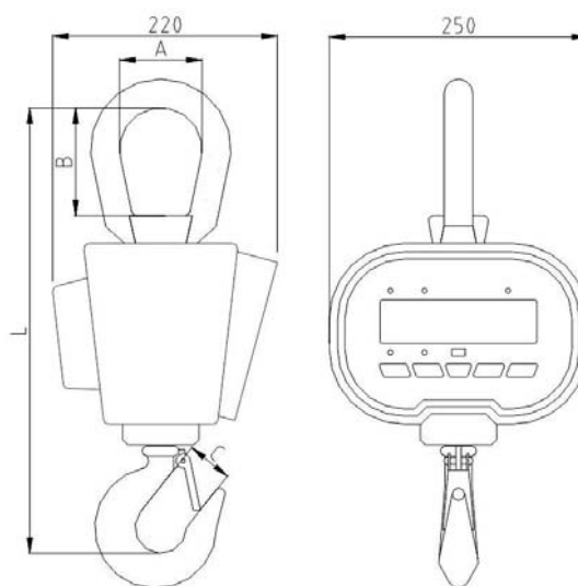
Dimensions (mm)
