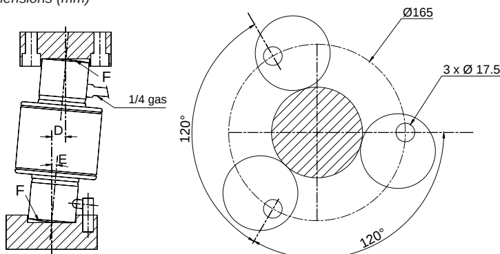
Dimensions (mm)
