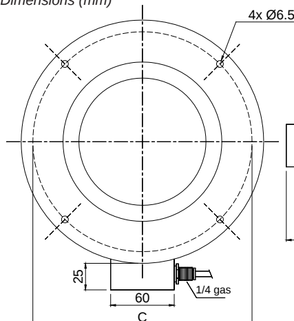
Dimensions (mm)
